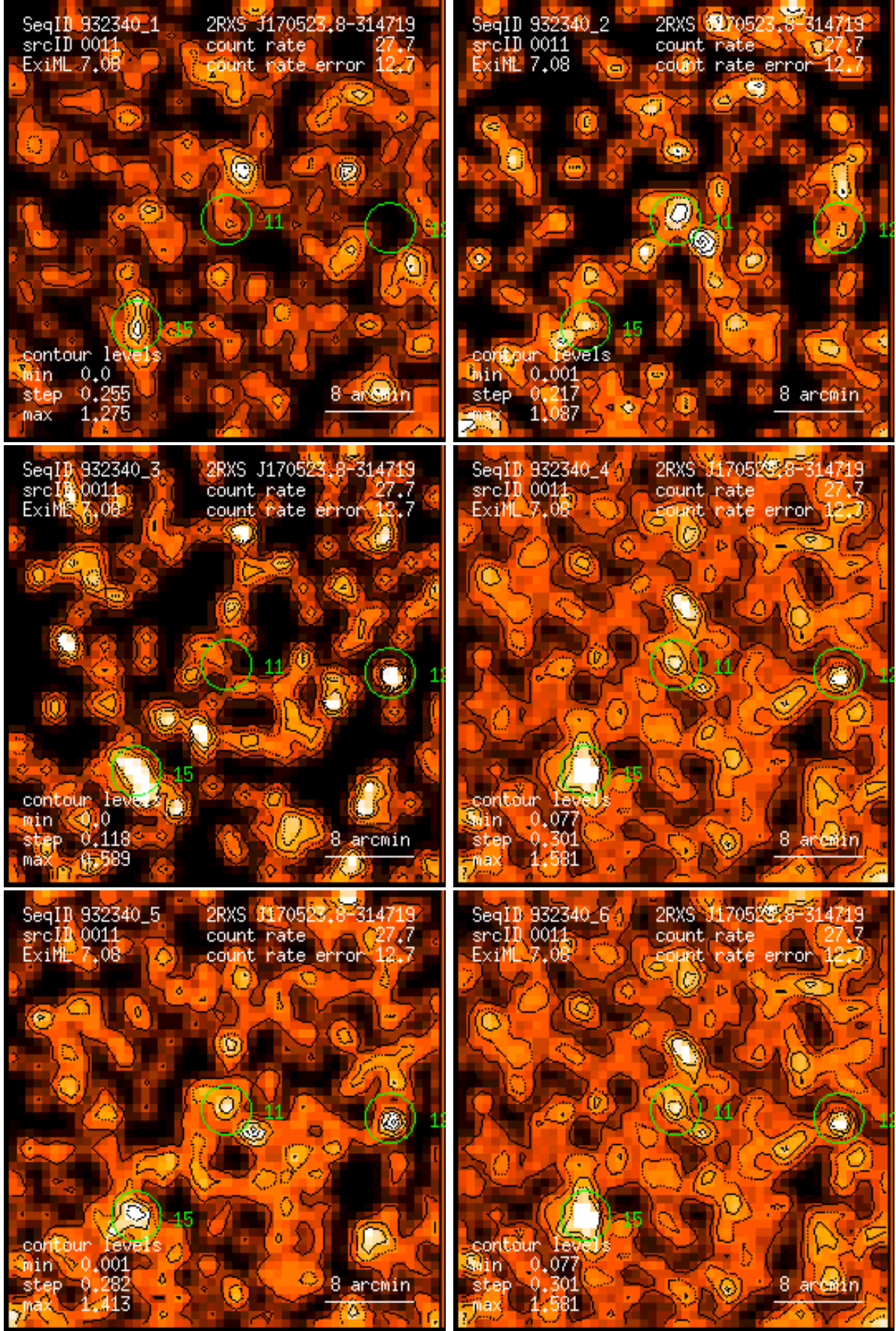
Figure 11: RASS 932340: detection 0011: band rate images, Gaussian filter: (1) PSPC channels 11 – 41, (2) 52 – 90, (3) 91 – 201, (4) 11 – 235, (5) 52 – 201, (6) 11 – 201. Broad band rates in counts/ks. Band rate contour levels in counts/ks/arcmin 2 .
