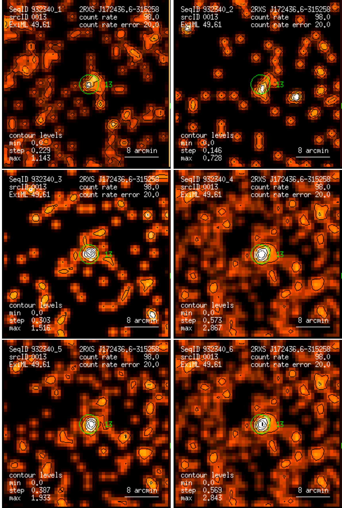
Figure 13: RASS 932340: detection 0013: band rate images, Gaussian filter: (1) PSPC channels 11 – 41, (2) 52 – 90, (3) 91 – 201, (4) 11 – 235, (5) 52 – 201, (6) 11 – 201. Broad band rates in counts/ks. Band rate contour levels in counts/ks/arcmin 2 .
