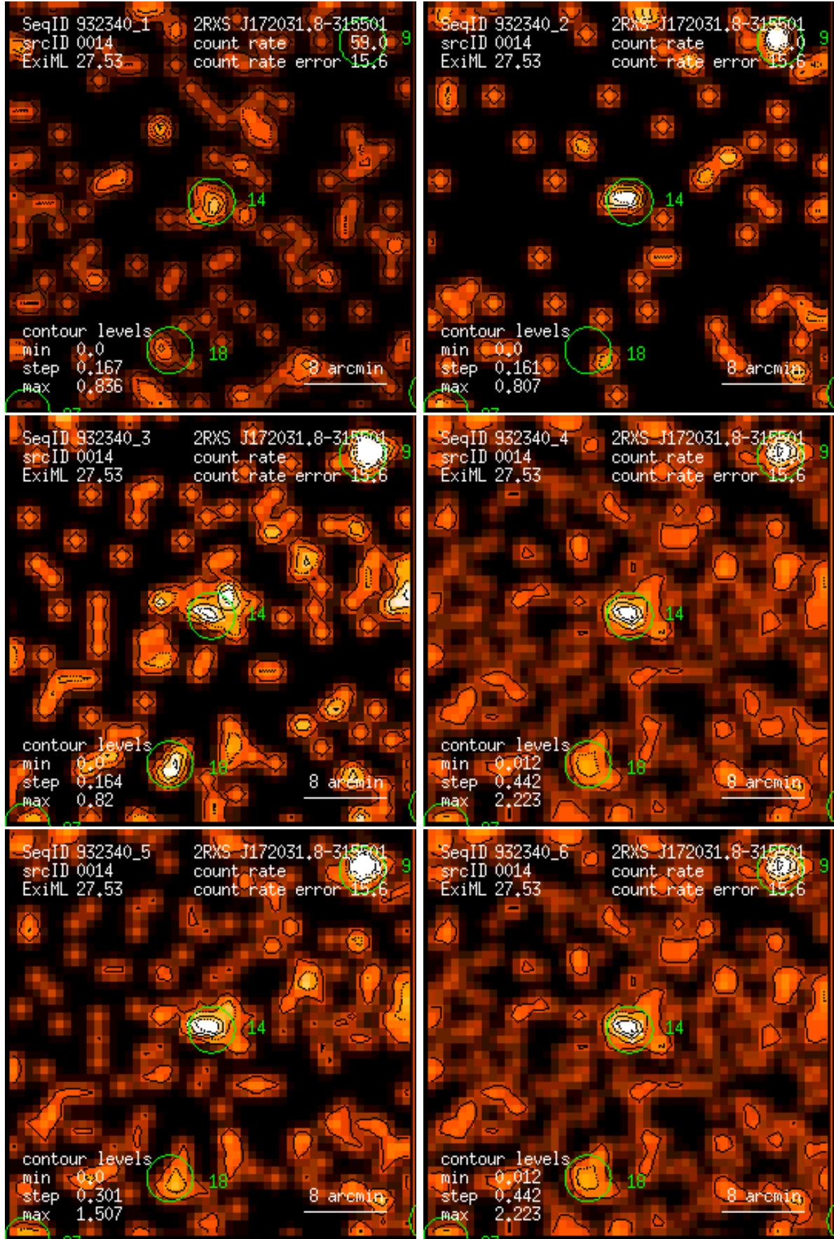
Figure 14: RASS 932340: detection 0014: band rate images, Gaussian filter: (1) PSPC channels 11 – 41, (2) 52 – 90, (3) 91 – 201, (4) 11 – 235, (5) 52 – 201, (6) 11 – 201. Broad band rates in counts/ks. Band rate contour levels in counts/ks/arcmin 2 .
