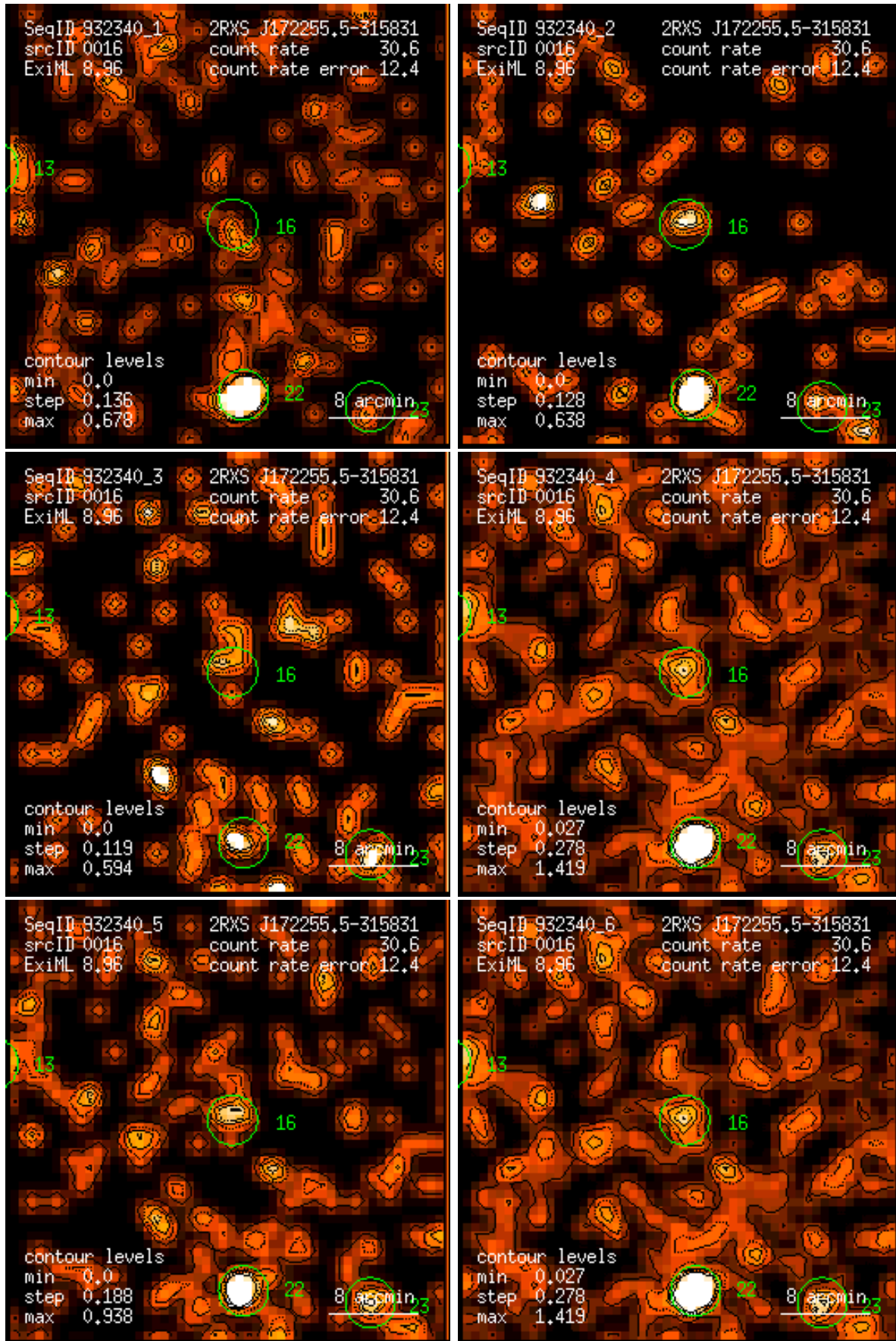
Figure 16: RASS 932340: detection 0016: band rate images, Gaussian filter: (1) PSPC channels 11 – 41, (2) 52 – 90, (3) 91 – 201, (4) 11 – 235, (5) 52 – 201, (6) 11 – 201. Broad band rates in counts/ks. Band rate contour levels in counts/ks/arcmin 2 .
