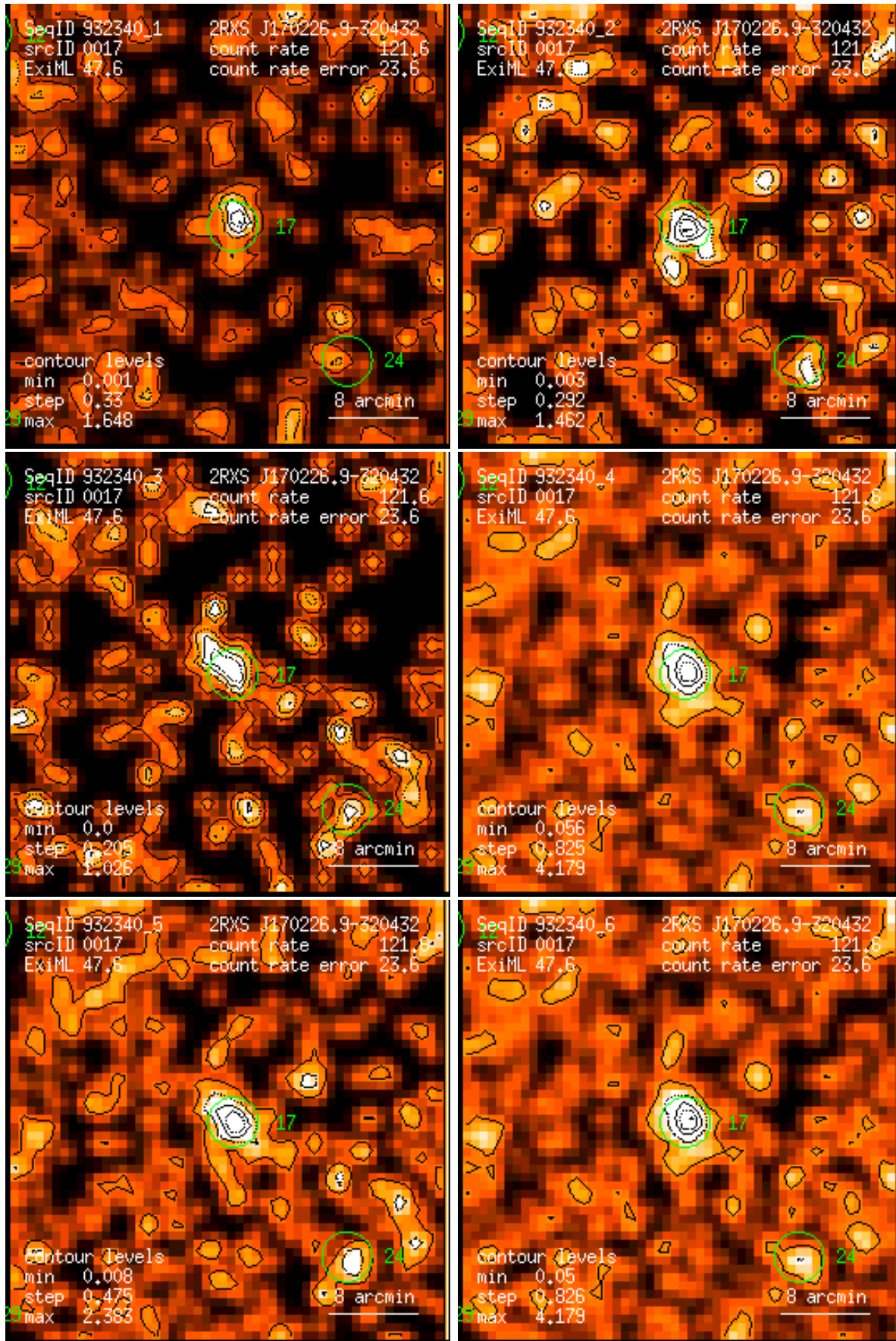
Figure 17: RASS 932340: detection 0017: band rate images, Gaussian filter: (1) PSPC channels 11 – 41, (2) 52 – 90, (3) 91 – 201, (4) 11 – 235, (5) 52 – 201, (6) 11 – 201. Broad band rates in counts/ks. Band rate contour levels in counts/ks/arcmin 2 .
