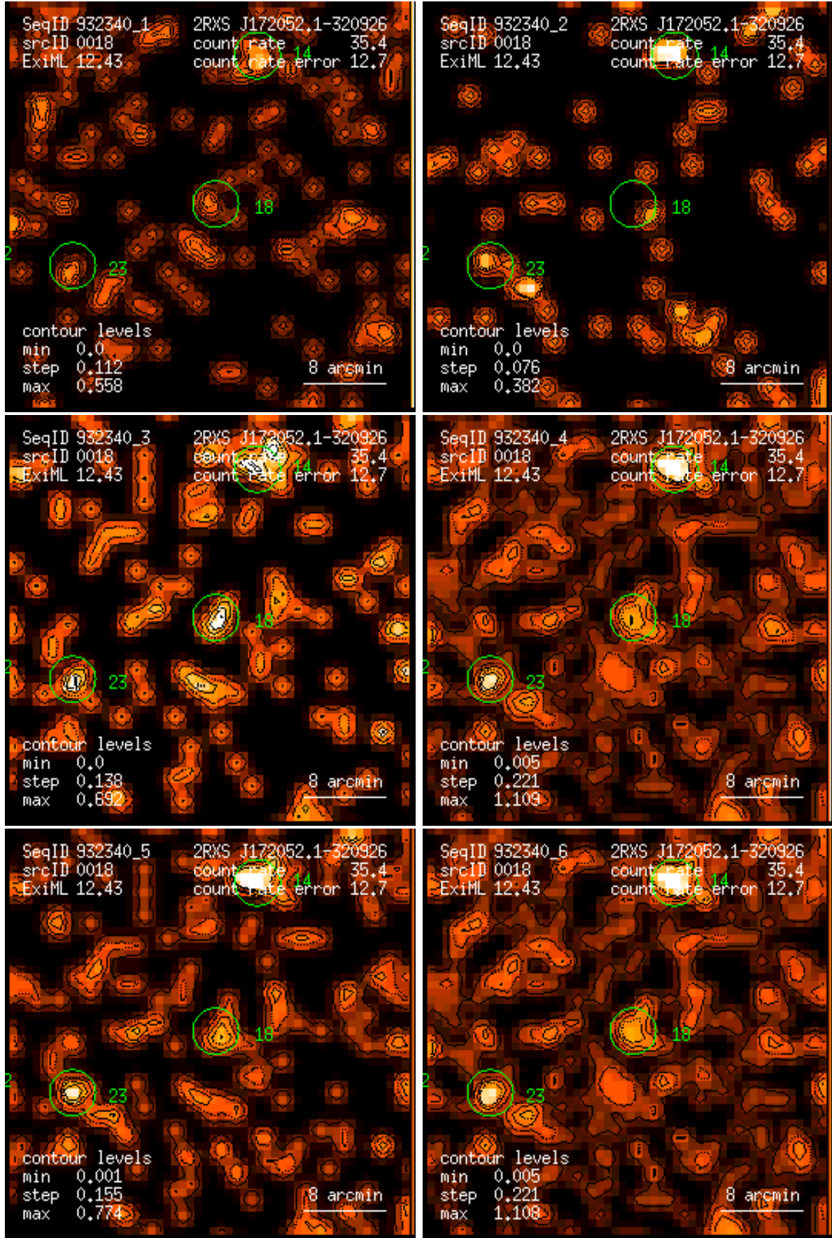
Figure 18: RASS 932340: detection 0018: band rate images, Gaussian filter: (1) PSPC channels 11 – 41, (2) 52 – 90, (3) 91 – 201, (4) 11 – 235, (5) 52 – 201, (6) 11 – 201. Broad band rates in counts/ks. Band rate contour levels in counts/ks/arcmin 2 .
