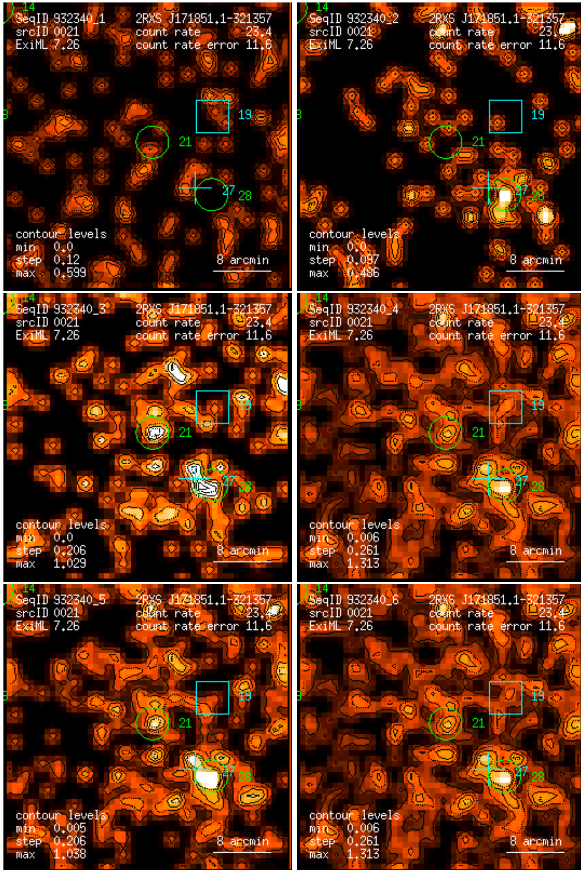
Figure 21: RASS 932340: detection 0021: band rate images, Gaussian filter: (1) PSPC channels 11 – 41, (2) 52 – 90, (3) 91 – 201, (4) 11 – 235, (5) 52 – 201, (6) 11 – 201. Broad band rates in counts/ks. Band rate contour levels in counts/ks/arcmin 2 .
