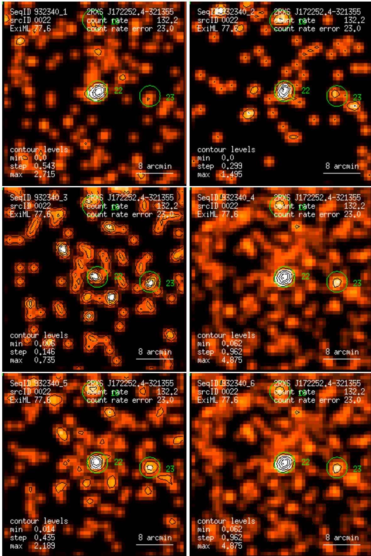
Figure 22: RASS 932340: detection 0022: band rate images, Gaussian filter: (1) PSPC channels 11 – 41, (2) 52 – 90, (3) 91 – 201, (4) 11 – 235, (5) 52 – 201, (6) 11 – 201. Broad band rates in counts/ks. Band rate contour levels in counts/ks/arcmin 2 .
