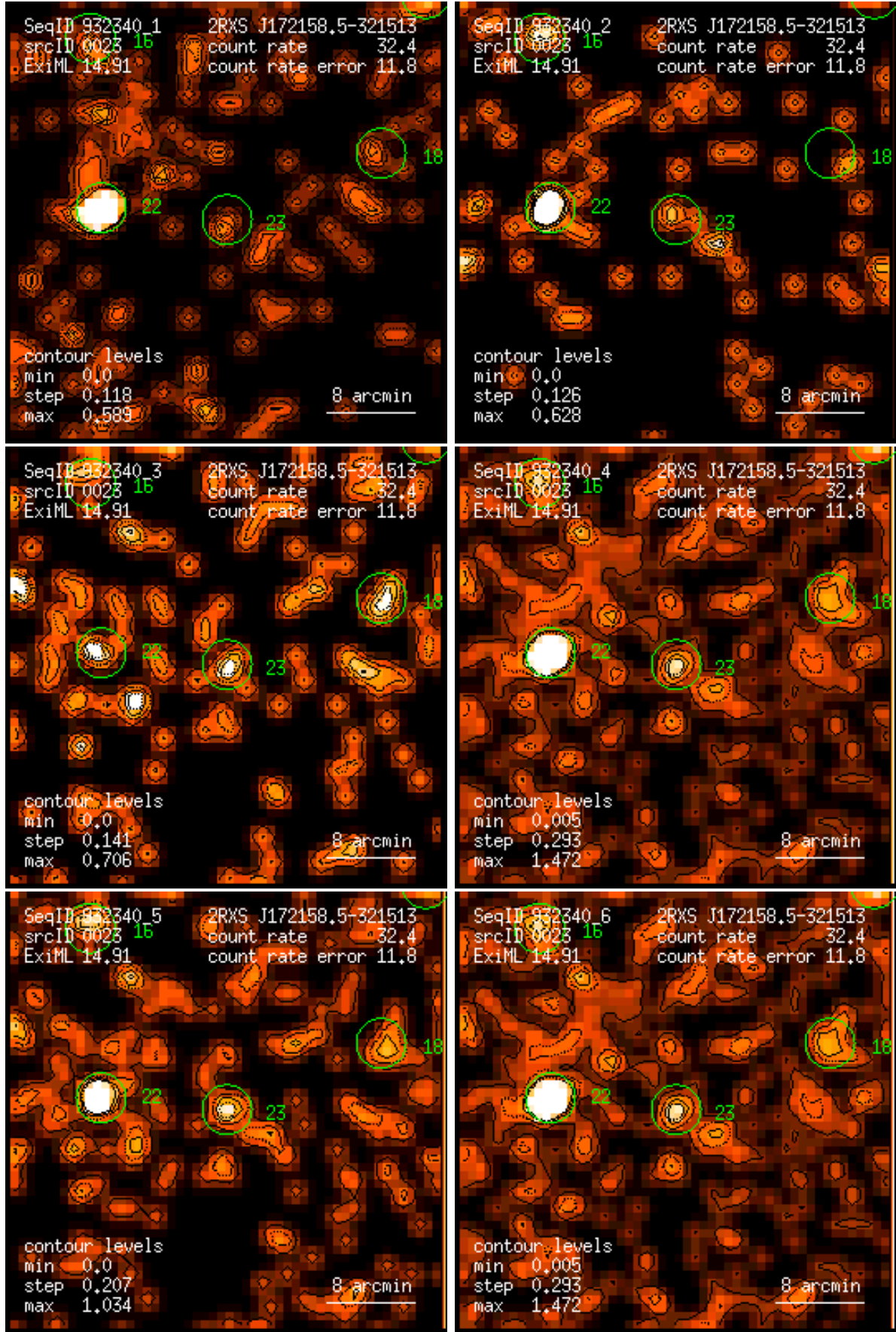
Figure 23: RASS 932340: detection 0023: band rate images, Gaussian filter: (1) PSPC channels 11 – 41, (2) 52 – 90, (3) 91 – 201, (4) 11 – 235, (5) 52 – 201, (6) 11 – 201. Broad band rates in counts/ks. Band rate contour levels in counts/ks/arcmin 2 .
