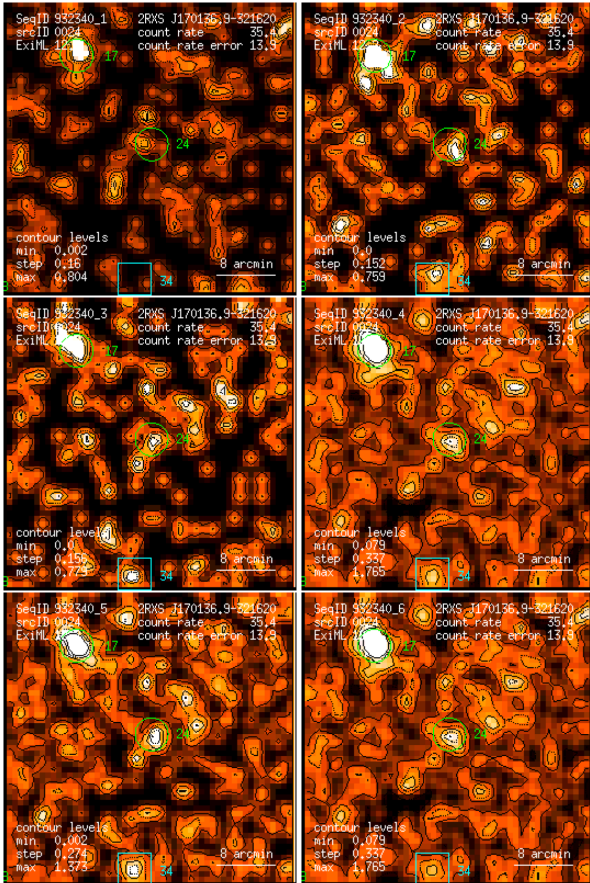
Figure 24: RASS 932340: detection 0024: band rate images, Gaussian filter: (1) PSPC channels 11 – 41, (2) 52 – 90, (3) 91 – 201, (4) 11 – 235, (5) 52 – 201, (6) 11 – 201. Broad band rates in counts/ks. Band rate contour levels in counts/ks/arcmin 2 .
