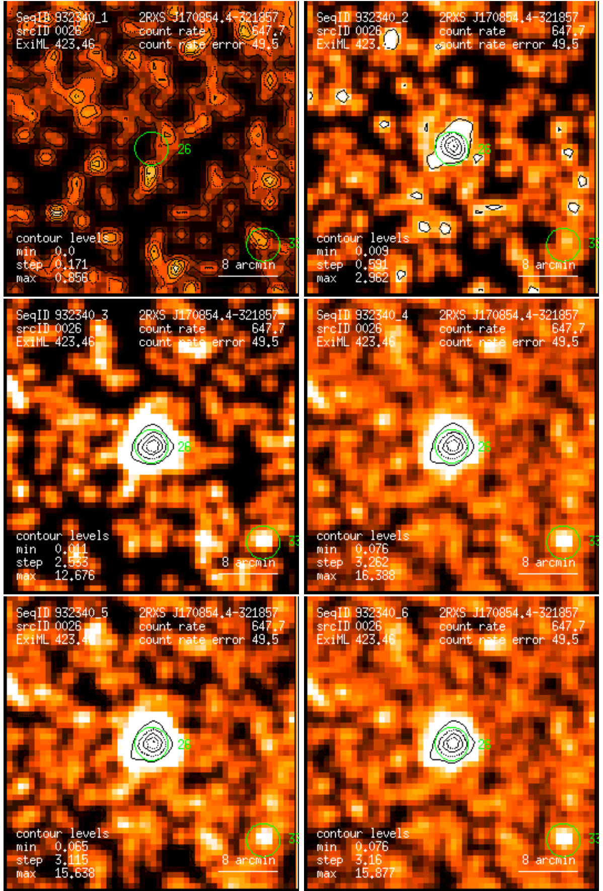
Figure 26: RASS 932340: detection 0026: band rate images, Gaussian filter: (1) PSPC channels 11 – 41, (2) 52 – 90, (3) 91 – 201, (4) 11 – 235, (5) 52 – 201, (6) 11 – 201. Broad band rates in counts/ks. Band rate contour levels in counts/ks/arcmin 2 .
