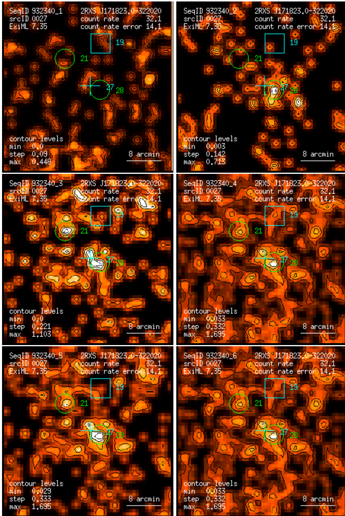
Figure 27: RASS 932340: detection 0027: band rate images, Gaussian filter: (1) PSPC channels 11 – 41, (2) 52 – 90, (3) 91 – 201, (4) 11 – 235, (5) 52 – 201, (6) 11 – 201. Broad band rates in counts/ks. Band rate contour levels in counts/ks/arcmin 2 .
