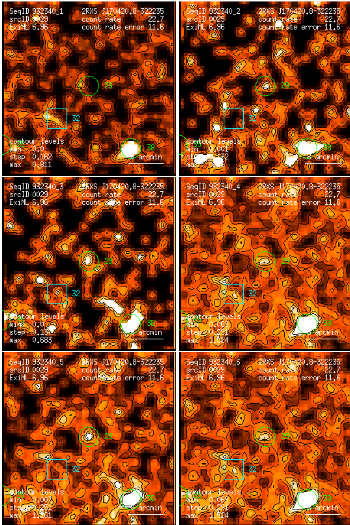
Figure 29: RASS 932340: detection 0029: band rate images, Gaussian filter: (1) PSPC channels 11 – 41, (2) 52 – 90, (3) 91 – 201, (4) 11 – 235, (5) 52 – 201, (6) 11 – 201. Broad band rates in counts/ks. Band rate contour levels in counts/ks/arcmin 2 .
