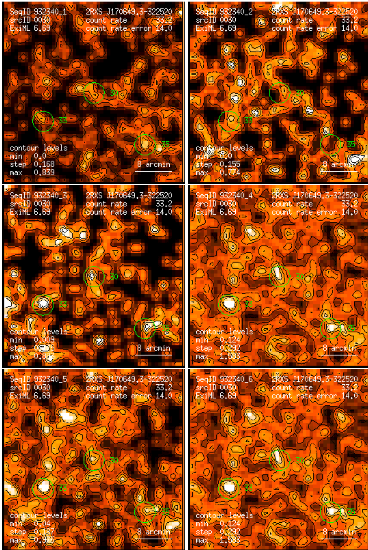
Figure 30: RASS 932340: detection 0030: band rate images, Gaussian filter: (1) PSPC channels 11 – 41, (2) 52 – 90, (3) 91 – 201, (4) 11 – 235, (5) 52 – 201, (6) 11 – 201. Broad band rates in counts/ks. Band rate contour levels in counts/ks/arcmin 2 .
