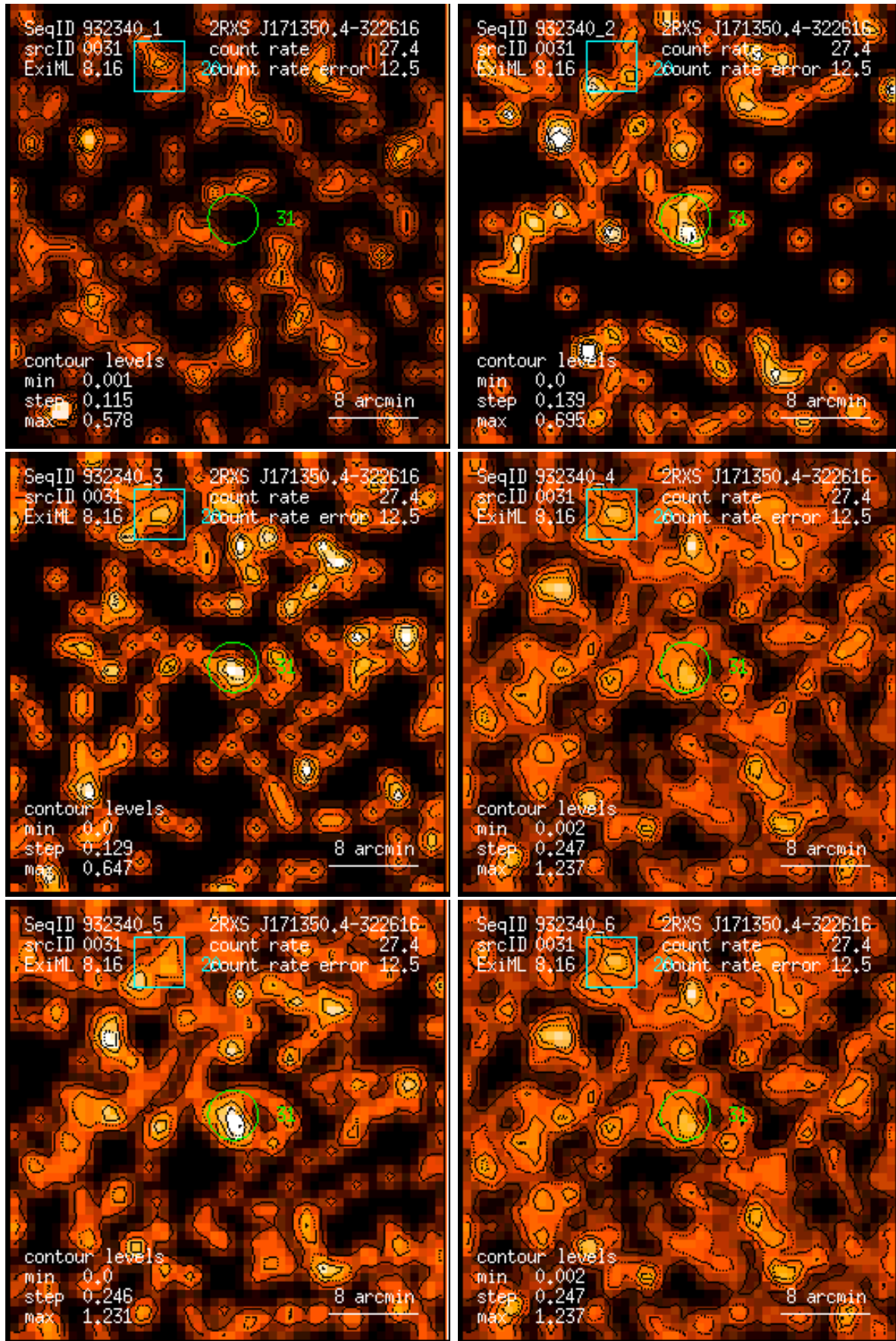
Figure 31: RASS 932340: detection 0031: band rate images, Gaussian filter: (1) PSPC channels 11 – 41, (2) 52 – 90, (3) 91 – 201, (4) 11 – 235, (5) 52 – 201, (6) 11 – 201. Broad band rates in counts/ks. Band rate contour levels in counts/ks/arcmin 2 .
