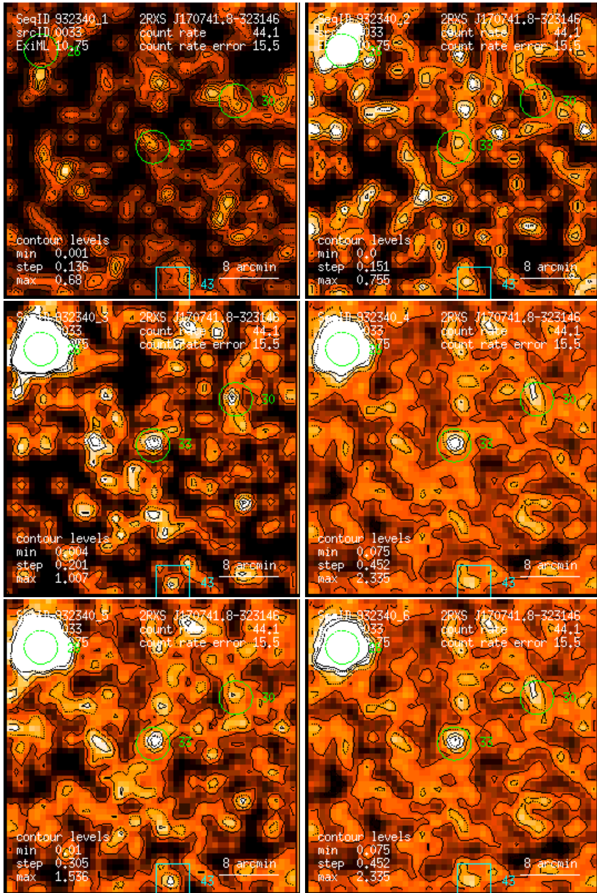
Figure 33: RASS 932340: detection 0033: band rate images, Gaussian filter: (1) PSPC channels 11 – 41, (2) 52 – 90, (3) 91 – 201, (4) 11 – 235, (5) 52 – 201, (6) 11 – 201. Broad band rates in counts/ks. Band rate contour levels in counts/ks/arcmin 2 .
