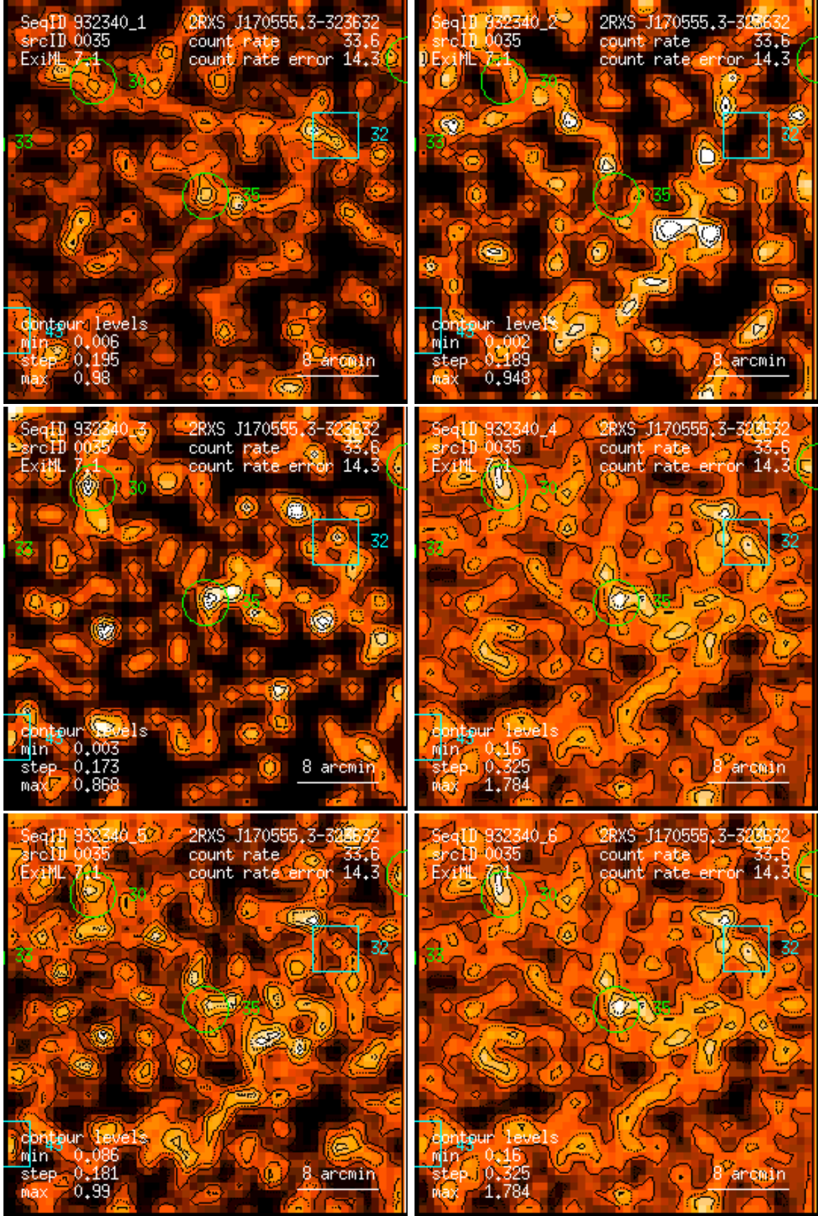
Figure 35: RASS 932340: detection 0035: band rate images, Gaussian filter: (1) PSPC channels 11 – 41, (2) 52 – 90, (3) 91 – 201, (4) 11 – 235, (5) 52 – 201, (6) 11 – 201. Broad band rates in counts/ks. Band rate contour levels in counts/ks/arcmin 2 .
