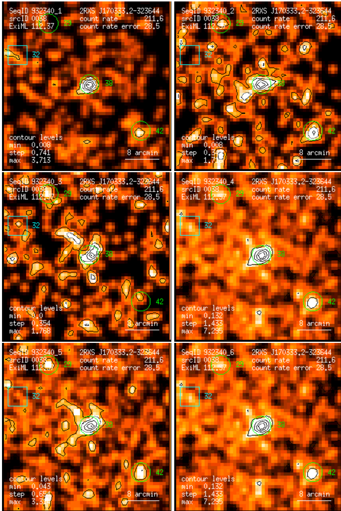
Figure 38: RASS 932340: detection 0038: band rate images, Gaussian filter: (1) PSPC channels 11 – 41, (2) 52 – 90, (3) 91 – 201, (4) 11 – 235, (5) 52 – 201, (6) 11 – 201. Broad band rates in counts/ks. Band rate contour levels in counts/ks/arcmin 2 .
