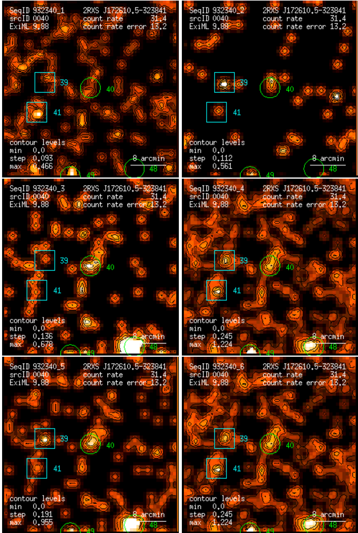
Figure 40: RASS 932340: detection 0040: band rate images, Gaussian filter: (1) PSPC channels 11 – 41, (2) 52 – 90, (3) 91 – 201, (4) 11 – 235, (5) 52 – 201, (6) 11 – 201. Broad band rates in counts/ks. Band rate contour levels in counts/ks/arcmin 2 .
