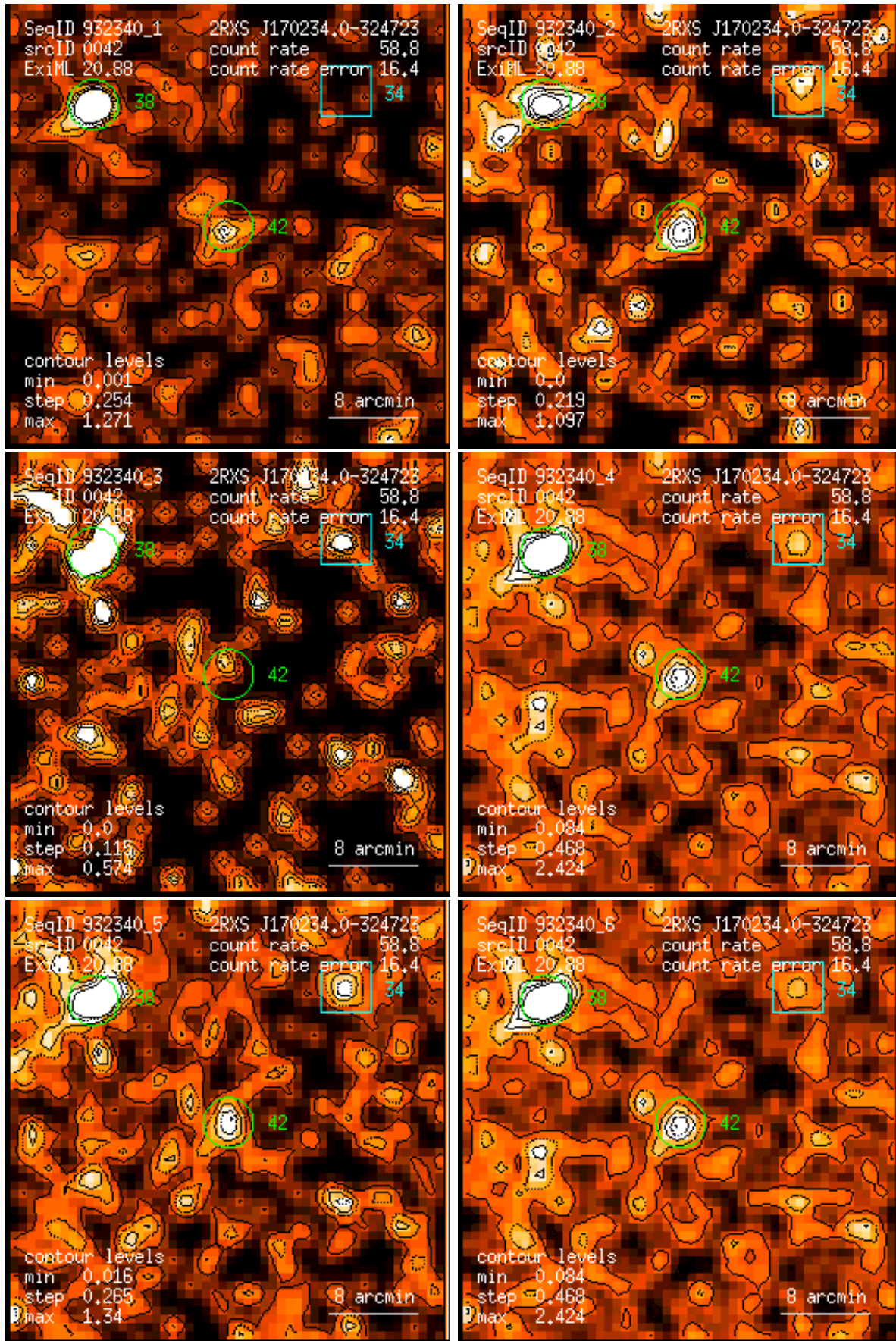
Figure 42: RASS 932340: detection 0042: band rate images, Gaussian filter: (1) PSPC channels 11 – 41, (2) 52 – 90, (3) 91 – 201, (4) 11 – 235, (5) 52 – 201, (6) 11 – 201. Broad band rates in counts/ks. Band rate contour levels in counts/ks/arcmin 2 .
