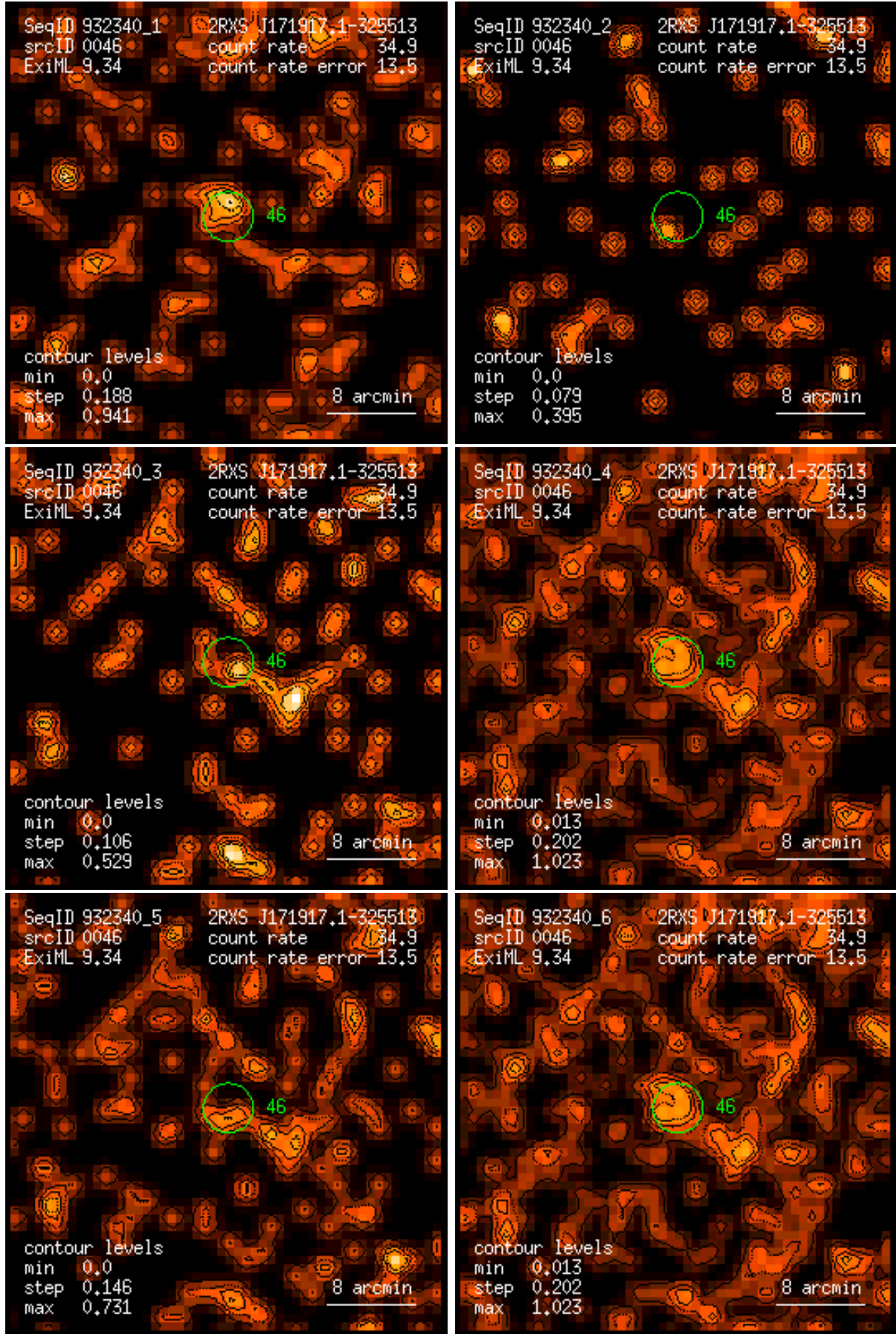
Figure 46: RASS 932340: detection 0046: band rate images, Gaussian filter: (1) PSPC channels 11 – 41, (2) 52 – 90, (3) 91 – 201, (4) 11 – 235, (5) 52 – 201, (6) 11 – 201. Broad band rates in counts/ks. Band rate contour levels in counts/ks/arcmin 2 .
