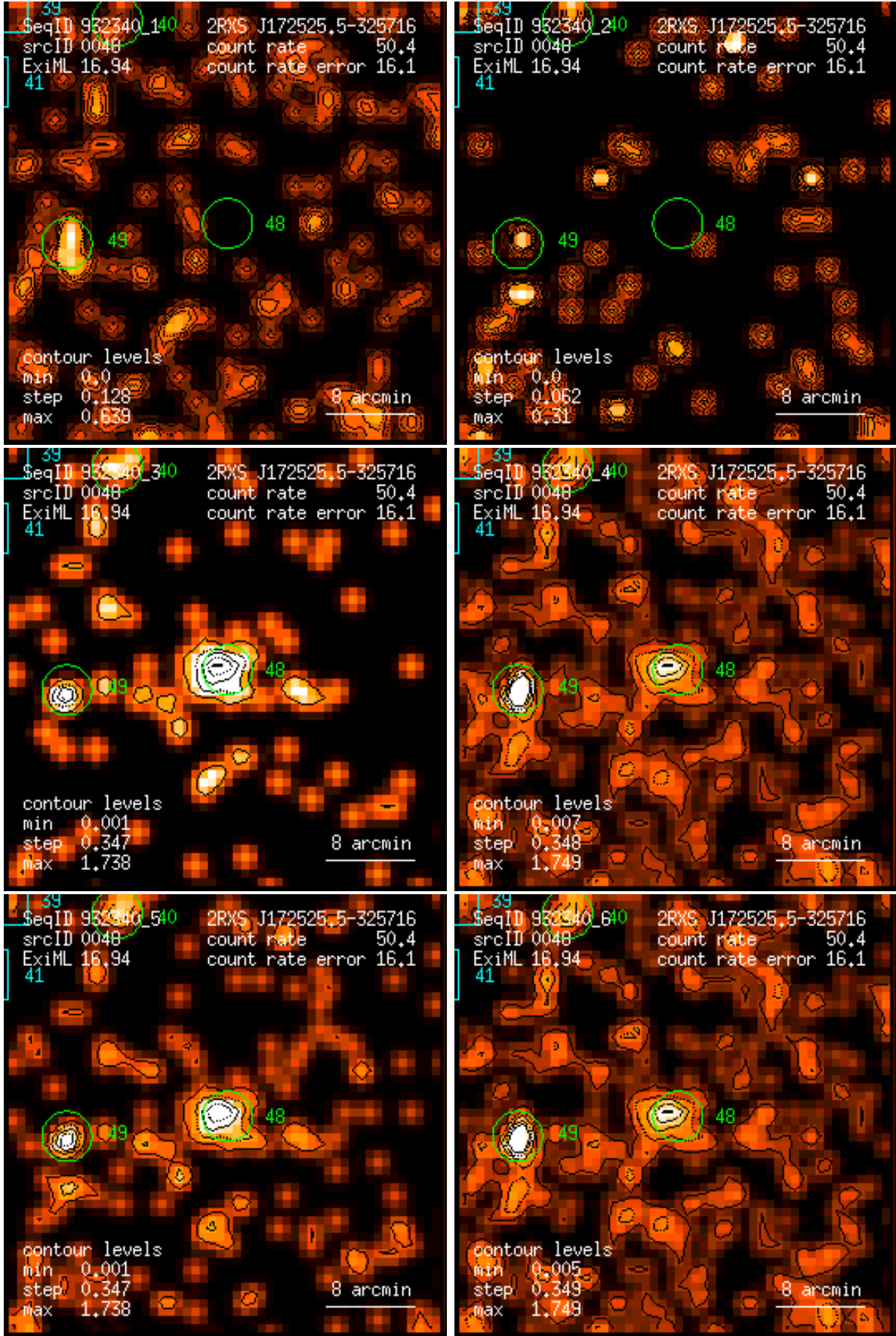
Figure 48: RASS 932340: detection 0048: band rate images, Gaussian filter: (1) PSPC channels 11 – 41, (2) 52 – 90, (3) 91 – 201, (4) 11 – 235, (5) 52 – 201, (6) 11 – 201. Broad band rates in counts/ks. Band rate contour levels in counts/ks/arcmin 2 .
