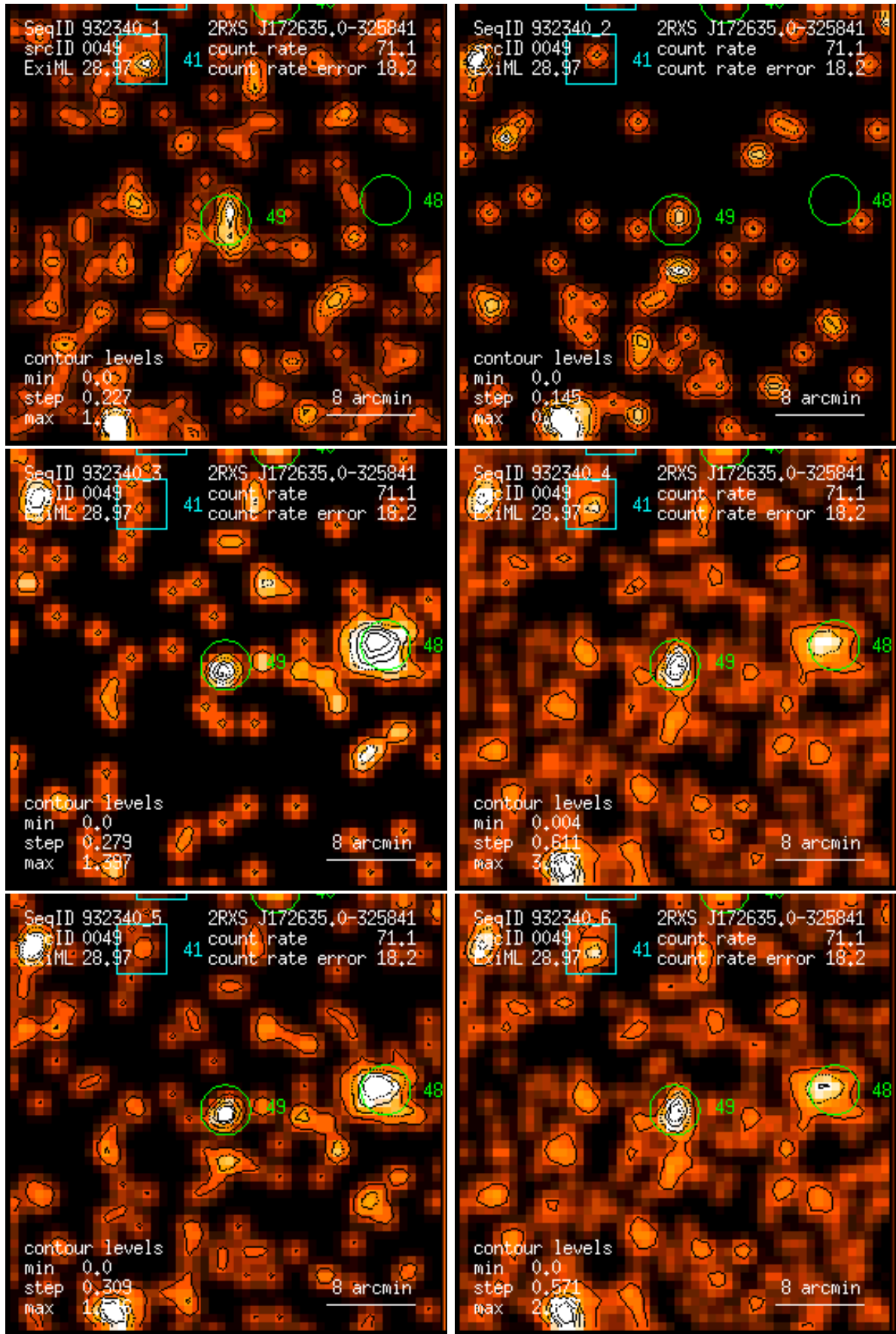
Figure 49: RASS 932340: detection 0049: band rate images, Gaussian filter: (1) PSPC channels 11 – 41, (2) 52 – 90, (3) 91 – 201, (4) 11 – 235, (5) 52 – 201, (6) 11 – 201. Broad band rates in counts/ks. Band rate contour levels in counts/ks/arcmin 2 .
