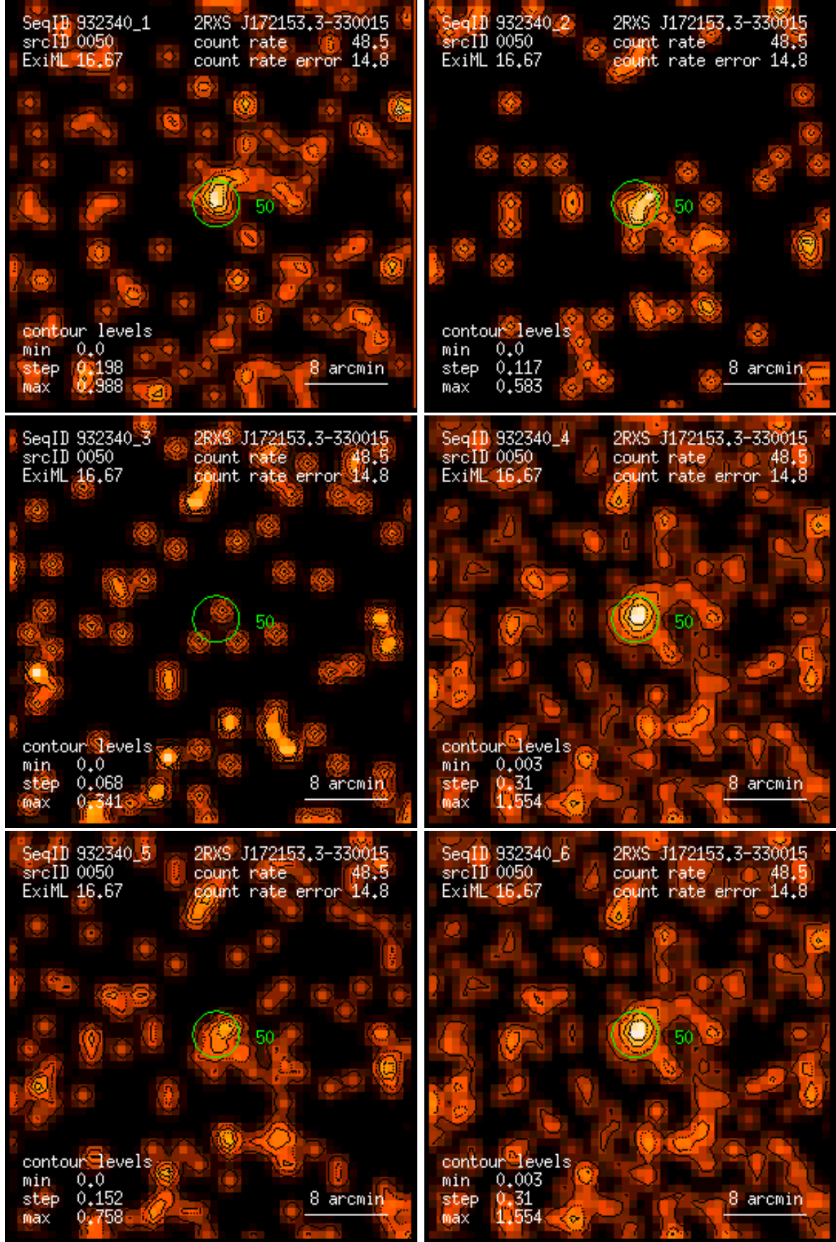
Figure 50: RASS 932340: detection 0050: band rate images, Gaussian filter: (1) PSPC channels 11 – 41, (2) 52 – 90, (3) 91 – 201, (4) 11 – 235, (5) 52 – 201, (6) 11 – 201. Broad band rates in counts/ks. Band rate contour levels in counts/ks/arcmin 2 .
