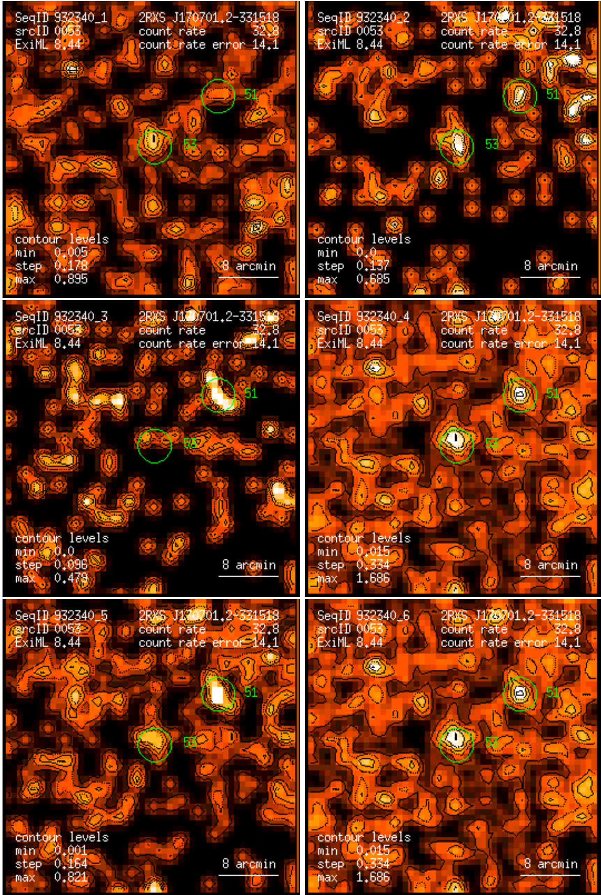
Figure 53: RASS 932340: detection 0053: band rate images, Gaussian filter: (1) PSPC channels 11 – 41, (2) 52 – 90, (3) 91 – 201, (4) 11 – 235, (5) 52 – 201, (6) 11 – 201. Broad band rates in counts/ks. Band rate contour levels in counts/ks/arcmin 2 .
