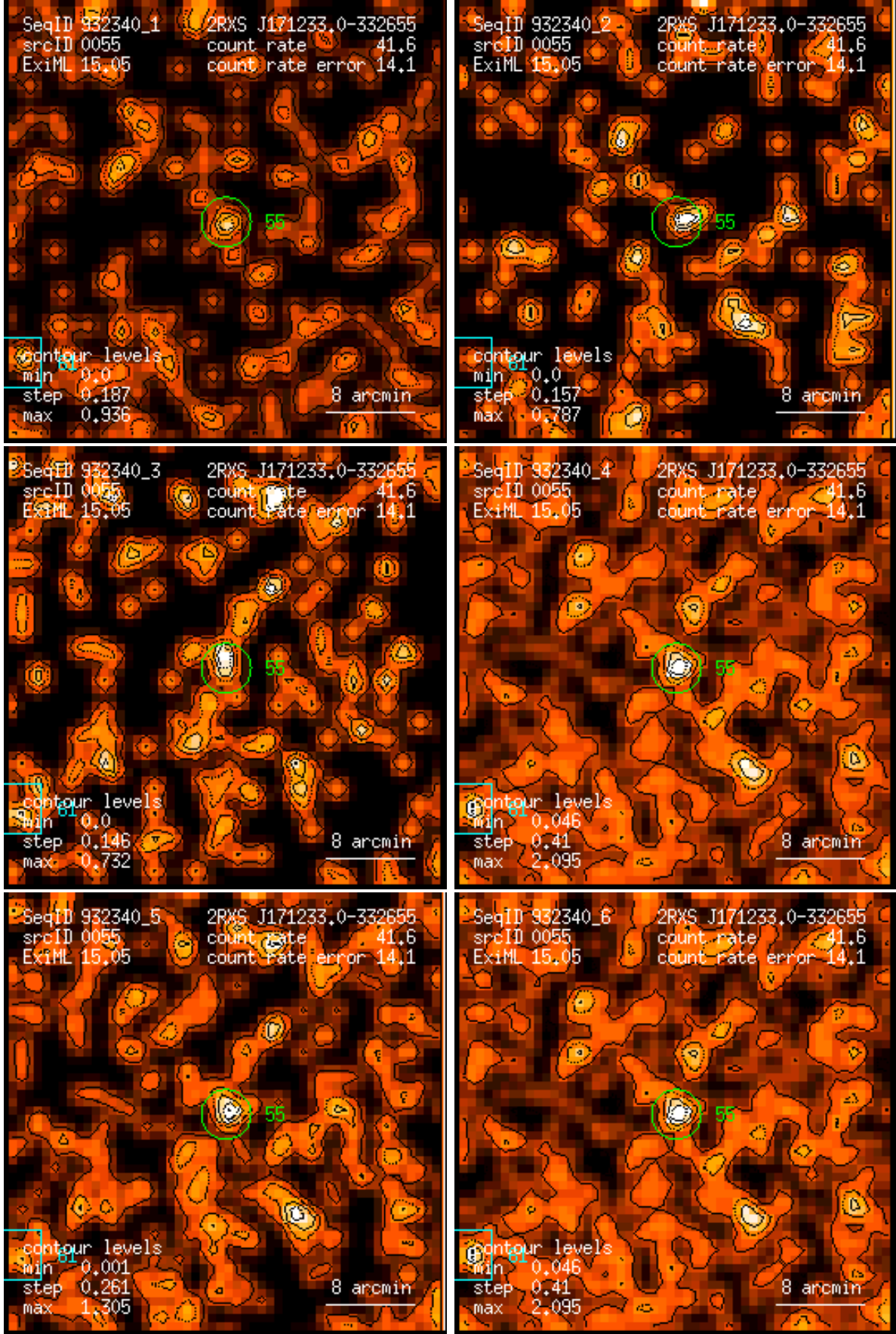
Figure 55: RASS 932340: detection 0055: band rate images, Gaussian filter: (1) PSPC channels 11 – 41, (2) 52 – 90, (3) 91 – 201, (4) 11 – 235, (5) 52 – 201, (6) 11 – 201. Broad band rates in counts/ks. Band rate contour levels in counts/ks/arcmin 2 .
