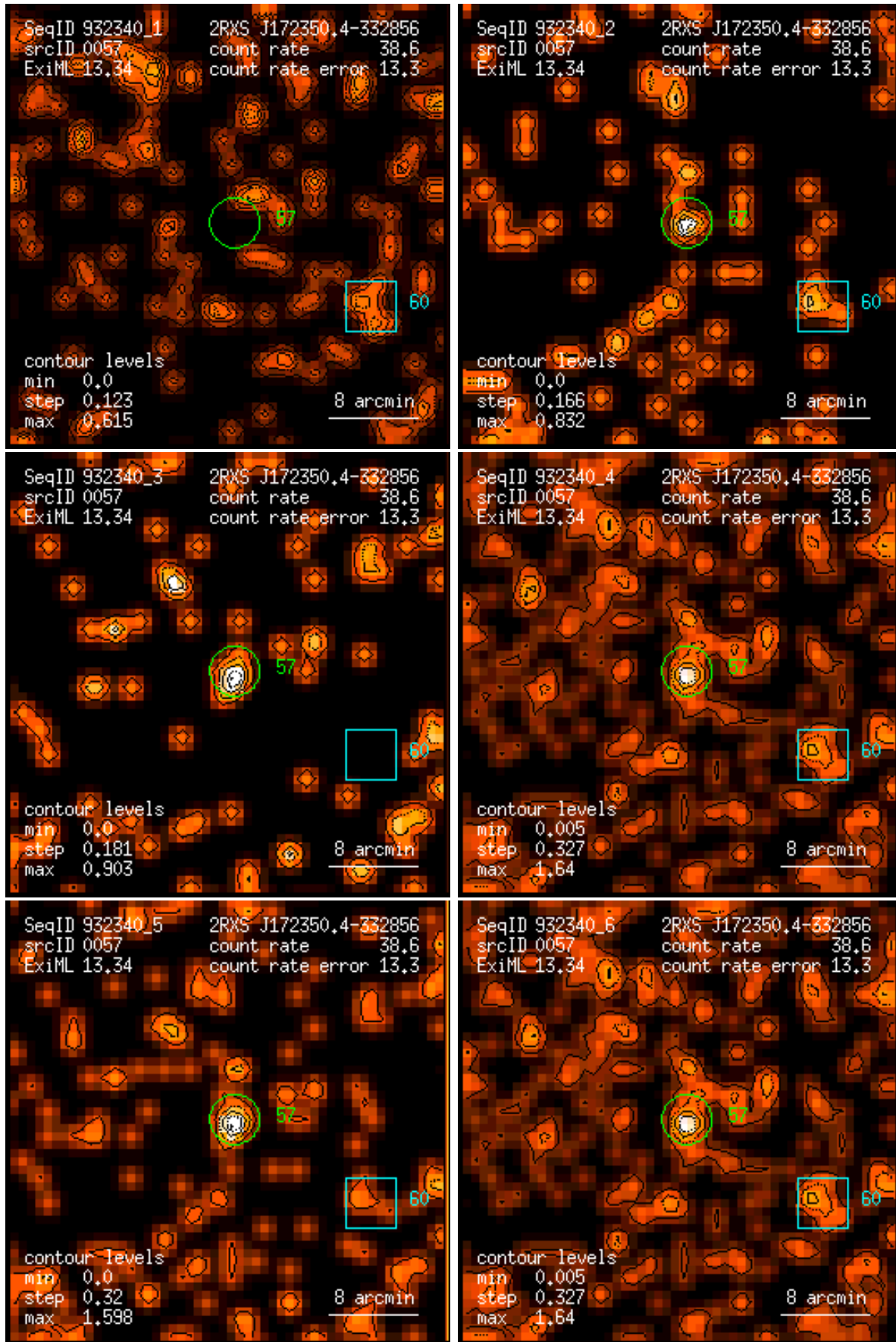
Figure 57: RASS 932340: detection 0057: band rate images, Gaussian filter: (1) PSPC channels 11 – 41, (2) 52 – 90, (3) 91 – 201, (4) 11 – 235, (5) 52 – 201, (6) 11 – 201. Broad band rates in counts/ks. Band rate contour levels in counts/ks/arcmin 2 .
