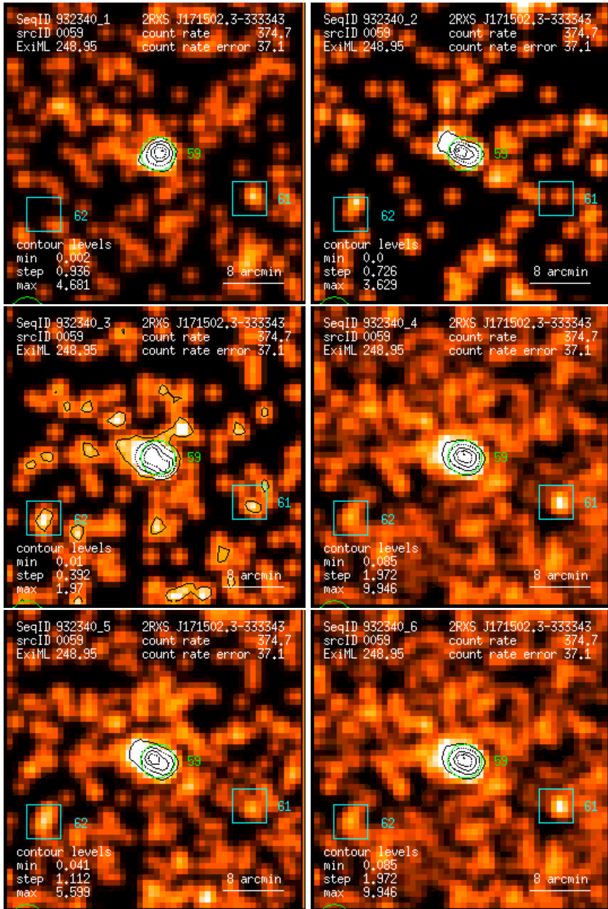
Figure 59: RASS 932340: detection 0059: band rate images, Gaussian filter: (1) PSPC channels 11 – 41, (2) 52 – 90, (3) 91 – 201, (4) 11 – 235, (5) 52 – 201, (6) 11 – 201. Broad band rates in counts/ks. Band rate contour levels in counts/ks/arcmin 2 .
