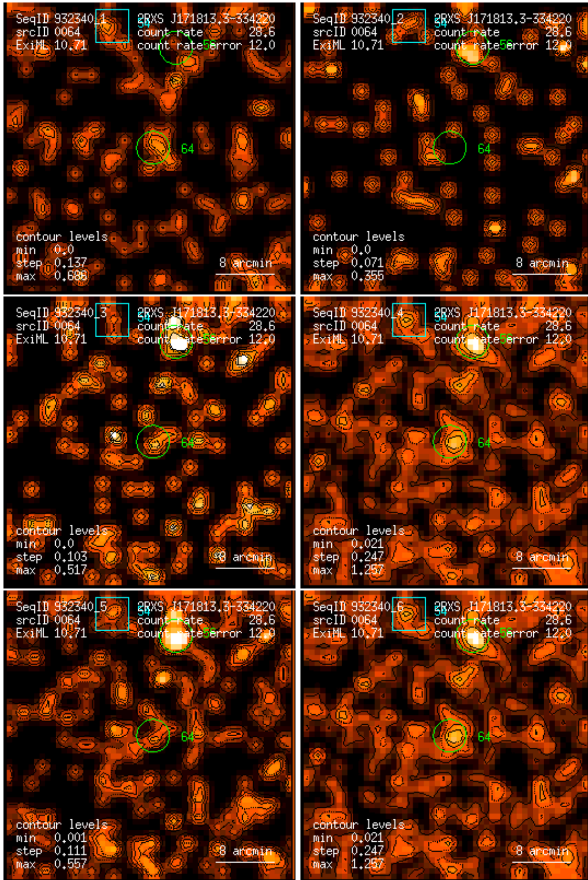
Figure 64: RASS 932340: detection 0064: band rate images, Gaussian filter: (1) PSPC channels 11 – 41, (2) 52 – 90, (3) 91 – 201, (4) 11 – 235, (5) 52 – 201, (6) 11 – 201. Broad band rates in counts/ks. Band rate contour levels in counts/ks/arcmin 2 .
