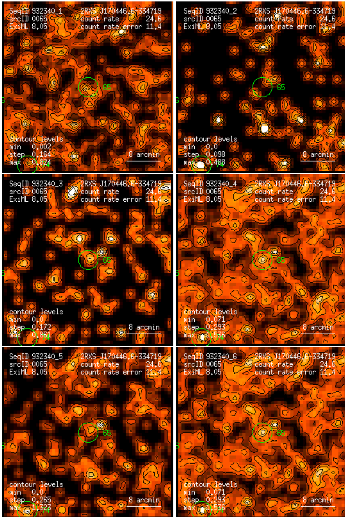
Figure 65: RASS 932340: detection 0065: band rate images, Gaussian filter: (1) PSPC channels 11 – 41, (2) 52 – 90, (3) 91 – 201, (4) 11 – 235, (5) 52 – 201, (6) 11 – 201. Broad band rates in counts/ks. Band rate contour levels in counts/ks/arcmin 2 .
