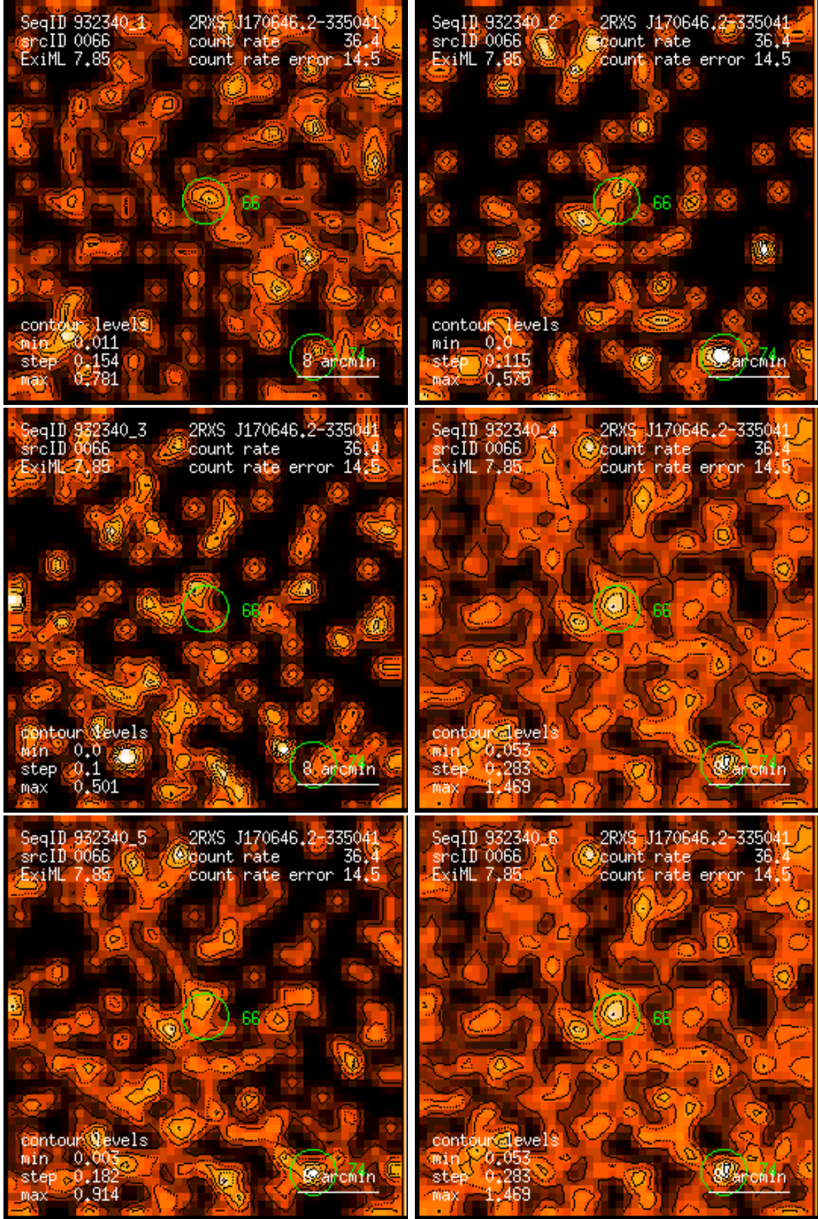
Figure 66: RASS 932340: detection 0066: band rate images, Gaussian filter: (1) PSPC channels 11 – 41, (2) 52 – 90, (3) 91 – 201, (4) 11 – 235, (5) 52 – 201, (6) 11 – 201. Broad band rates in counts/ks. Band rate contour levels in counts/ks/arcmin 2 .
