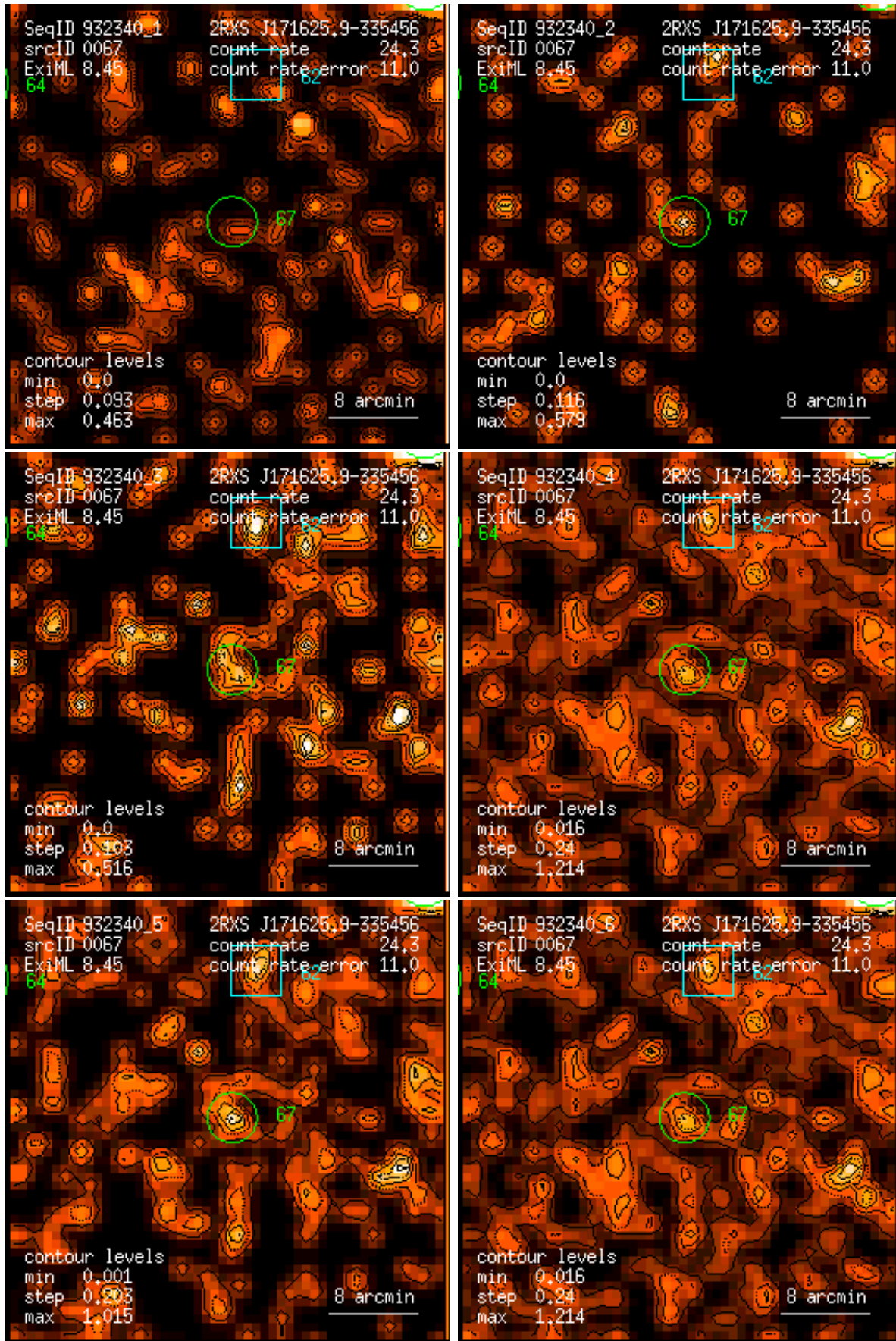
Figure 67: RASS 932340: detection 0067: band rate images, Gaussian filter: (1) PSPC channels 11 – 41, (2) 52 – 90, (3) 91 – 201, (4) 11 – 235, (5) 52 – 201, (6) 11 – 201. Broad band rates in counts/ks. Band rate contour levels in counts/ks/arcmin 2 .
