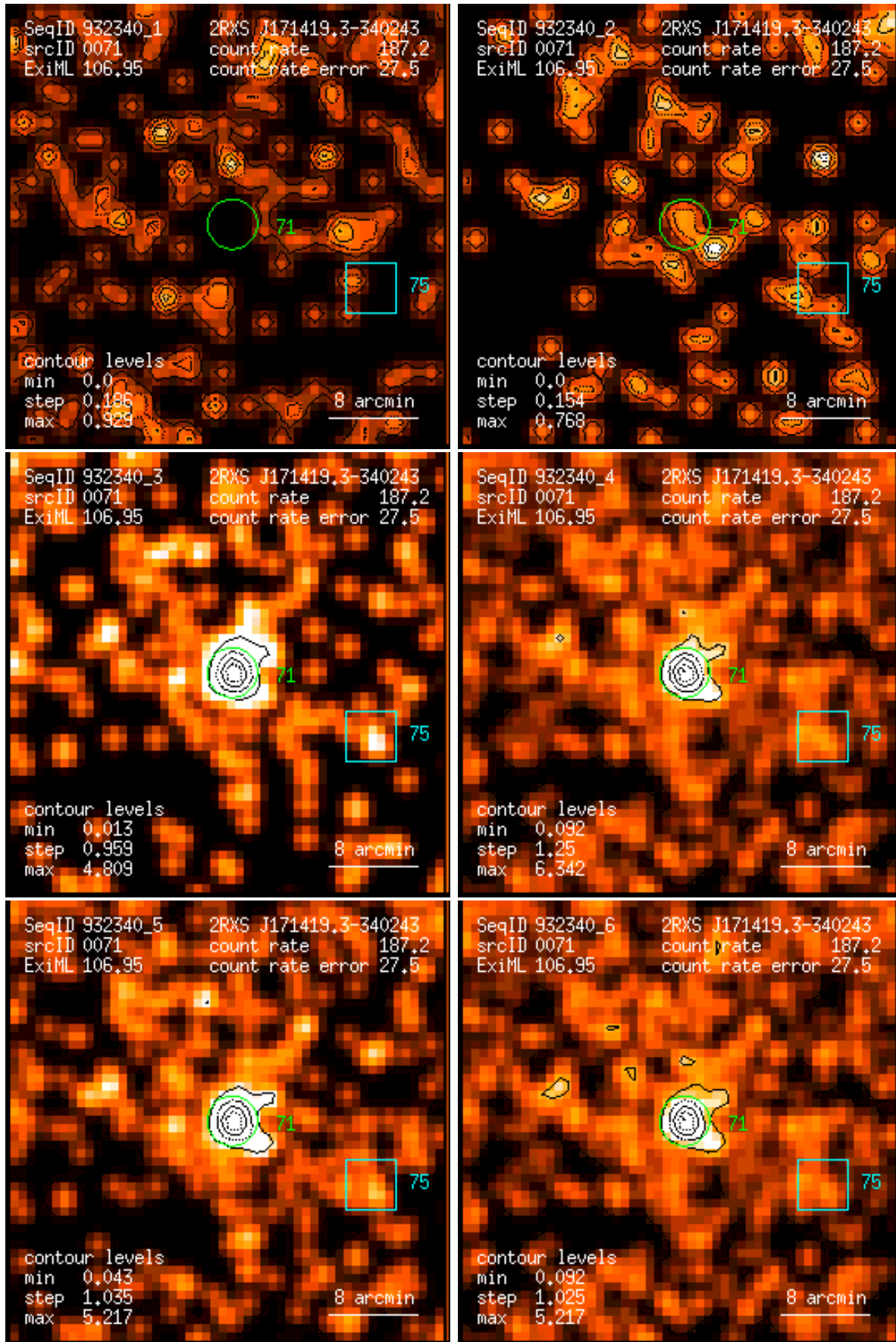
Figure 71: RASS 932340: detection 0071: band rate images, Gaussian filter: (1) PSPC channels 11 – 41, (2) 52 – 90, (3) 91 – 201, (4) 11 – 235, (5) 52 – 201, (6) 11 – 201. Broad band rates in counts/ks. Band rate contour levels in counts/ks/arcmin 2 .
