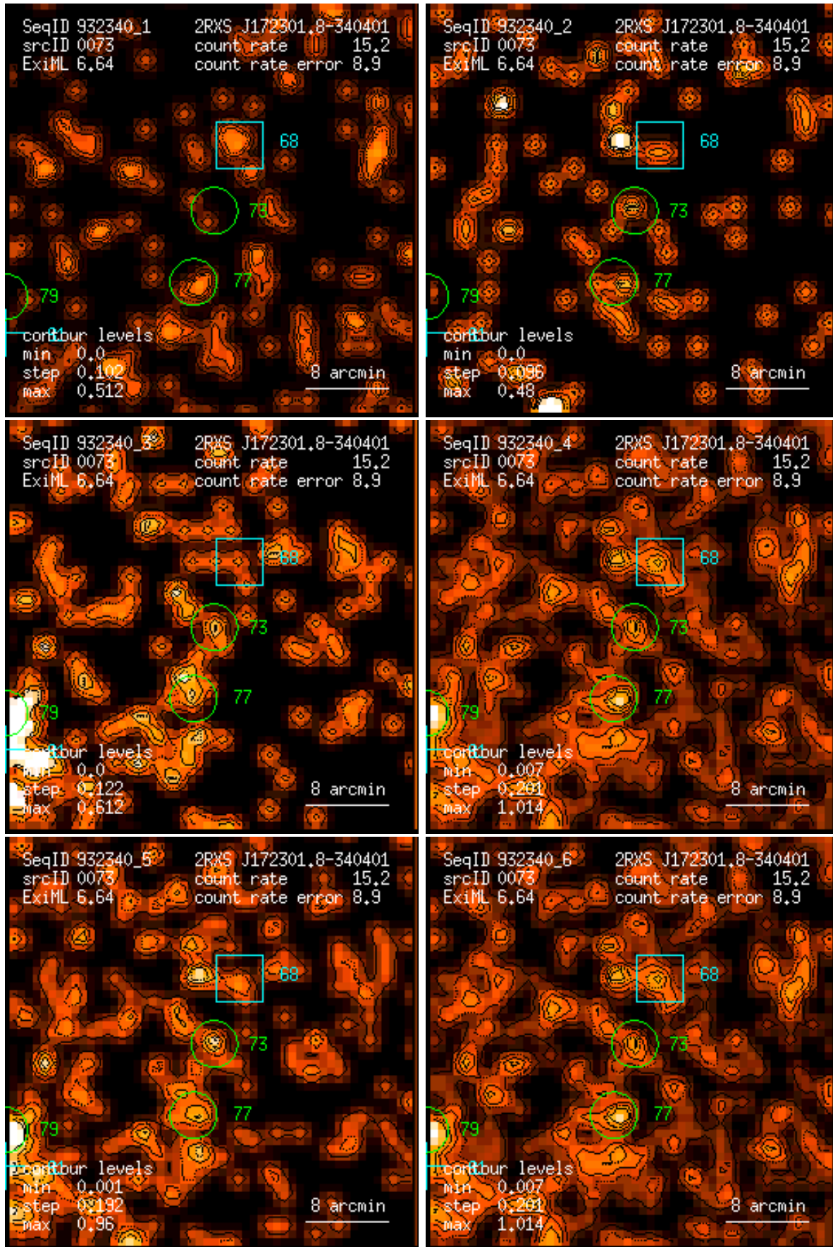
Figure 73: RASS 932340: detection 0073: band rate images, Gaussian filter: (1) PSPC channels 11 – 41, (2) 52 – 90, (3) 91 – 201, (4) 11 – 235, (5) 52 – 201, (6) 11 – 201. Broad band rates in counts/ks. Band rate contour levels in counts/ks/arcmin 2 .
