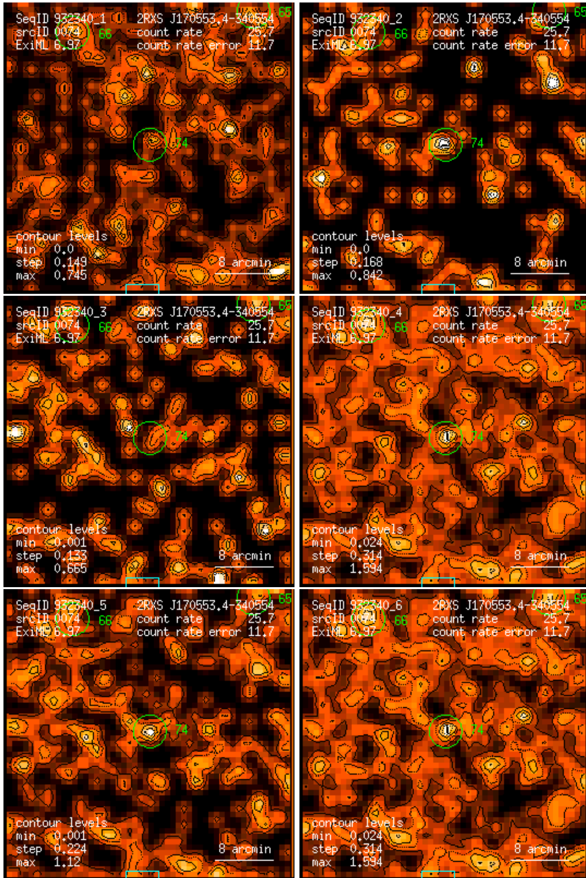
Figure 74: RASS 932340: detection 0074: band rate images, Gaussian filter: (1) PSPC channels 11 – 41, (2) 52 – 90, (3) 91 – 201, (4) 11 – 235, (5) 52 – 201, (6) 11 – 201. Broad band rates in counts/ks. Band rate contour levels in counts/ks/arcmin 2 .
