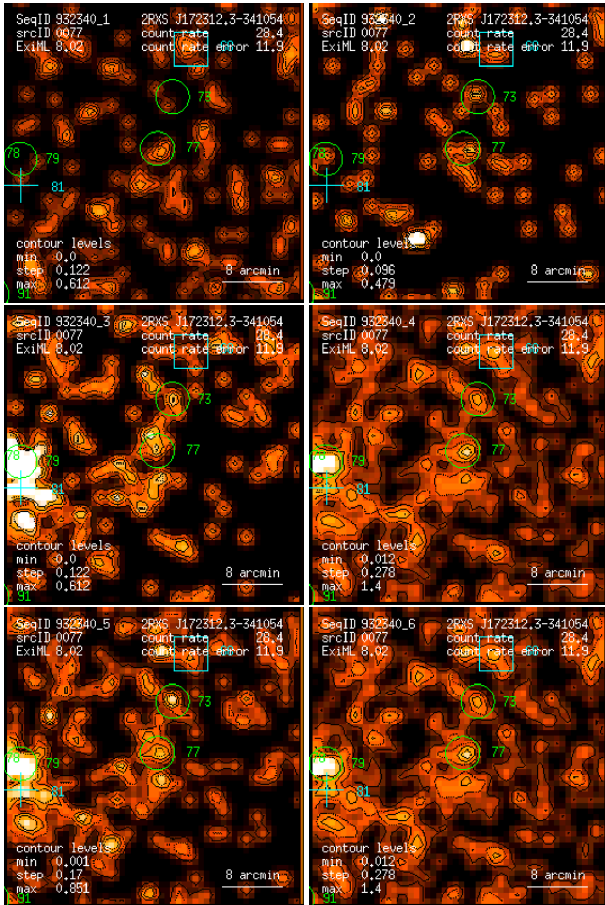
Figure 77: RASS 932340: detection 0077: band rate images, Gaussian filter: (1) PSPC channels 11 – 41, (2) 52 – 90, (3) 91 – 201, (4) 11 – 235, (5) 52 – 201, (6) 11 – 201. Broad band rates in counts/ks. Band rate contour levels in counts/ks/arcmin 2 .
