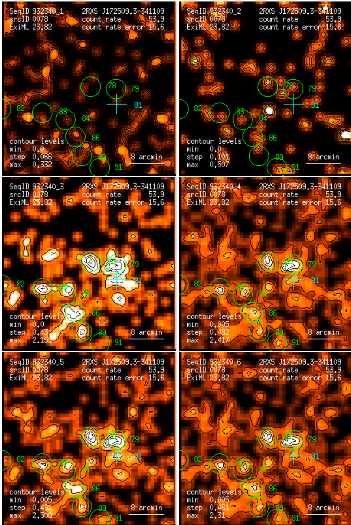
Figure 78: RASS 932340: detection 0078: band rate images, Gaussian filter: (1) PSPC channels 11 – 41, (2) 52 – 90, (3) 91 – 201, (4) 11 – 235, (5) 52 – 201, (6) 11 – 201. Broad band rates in counts/ks. Band rate contour levels in counts/ks/arcmin 2 .
