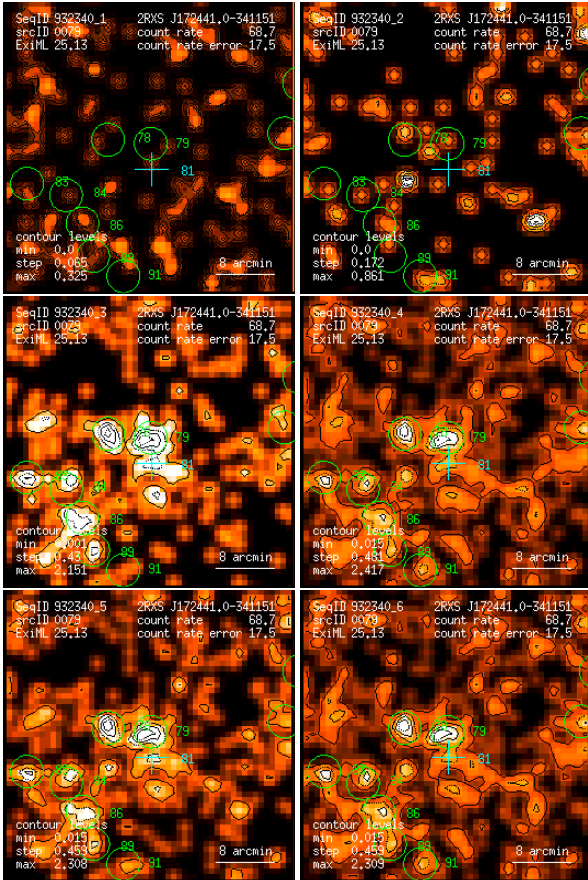
Figure 79: RASS 932340: detection 0079: band rate images, Gaussian filter: (1) PSPC channels 11 – 41, (2) 52 – 90, (3) 91 – 201, (4) 11 – 235, (5) 52 – 201, (6) 11 – 201. Broad band rates in counts/ks. Band rate contour levels in counts/ks/arcmin 2 .
