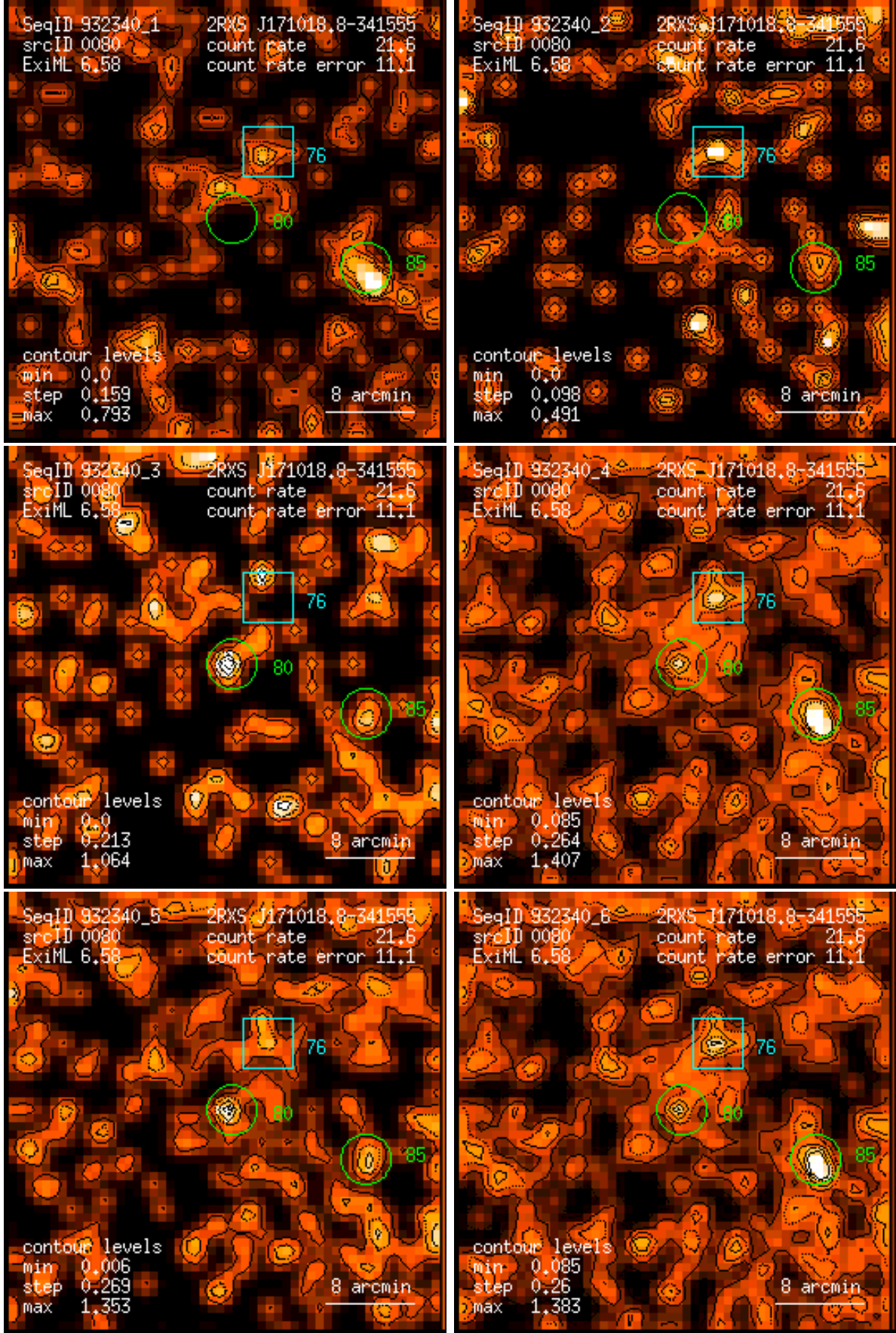
Figure 80: RASS 932340: detection 0080: band rate images, Gaussian filter: (1) PSPC channels 11 – 41, (2) 52 – 90, (3) 91 – 201, (4) 11 – 235, (5) 52 – 201, (6) 11 – 201. Broad band rates in counts/ks. Band rate contour levels in counts/ks/arcmin 2 .
