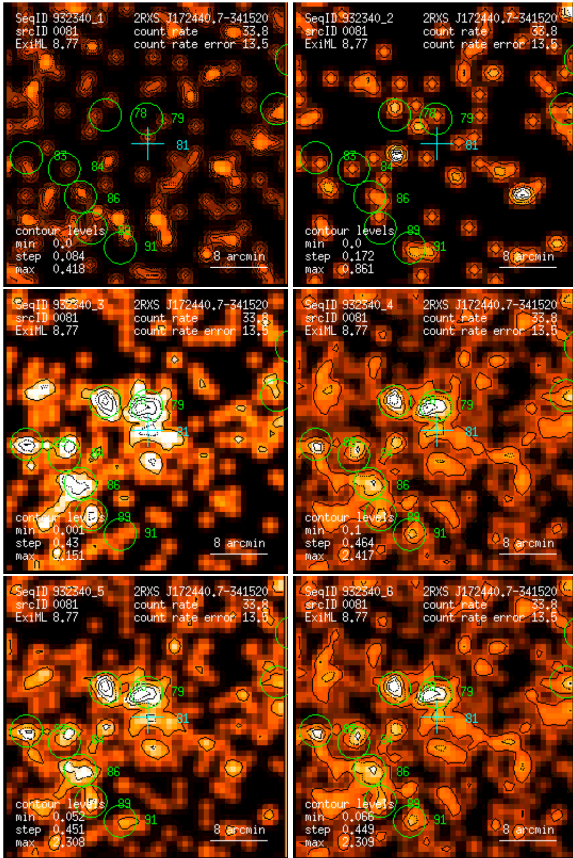
Figure 81: RASS 932340: detection 0081: band rate images, Gaussian filter: (1) PSPC channels 11 – 41, (2) 52 – 90, (3) 91 – 201, (4) 11 – 235, (5) 52 – 201, (6) 11 – 201. Broad band rates in counts/ks. Band rate contour levels in counts/ks/arcmin 2 .
