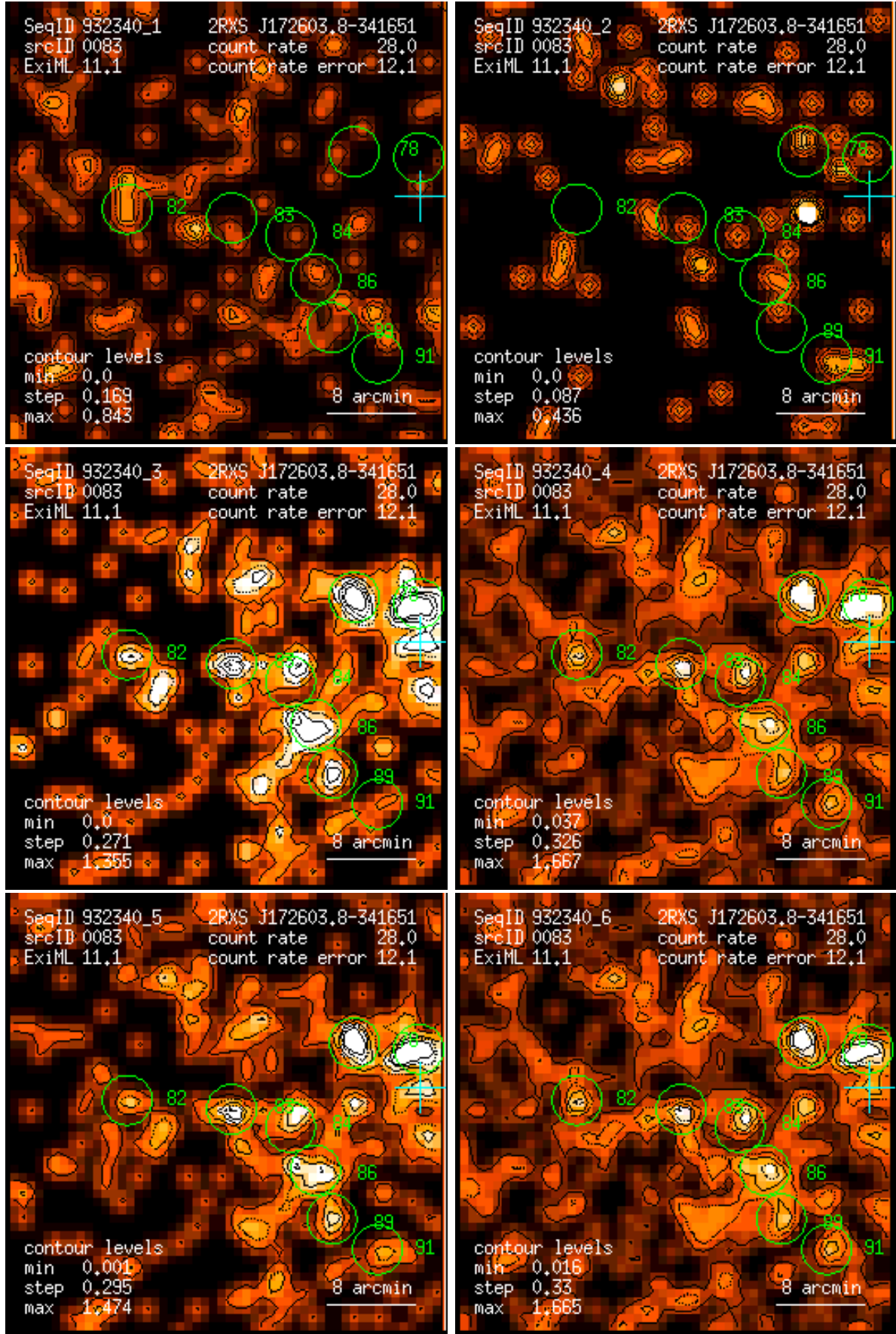
Figure 83: RASS 932340: detection 0083: band rate images, Gaussian filter: (1) PSPC channels 11 – 41, (2) 52 – 90, (3) 91 – 201, (4) 11 – 235, (5) 52 – 201, (6) 11 – 201. Broad band rates in counts/ks. Band rate contour levels in counts/ks/arcmin 2 .
