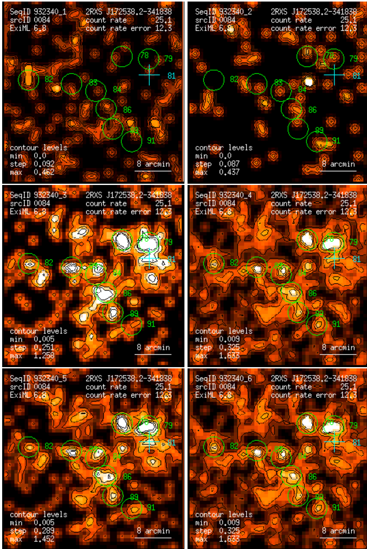
Figure 84: RASS 932340: detection 0084: band rate images, Gaussian filter: (1) PSPC channels 11 – 41, (2) 52 – 90, (3) 91 – 201, (4) 11 – 235, (5) 52 – 201, (6) 11 – 201. Broad band rates in counts/ks. Band rate contour levels in counts/ks/arcmin 2 .
