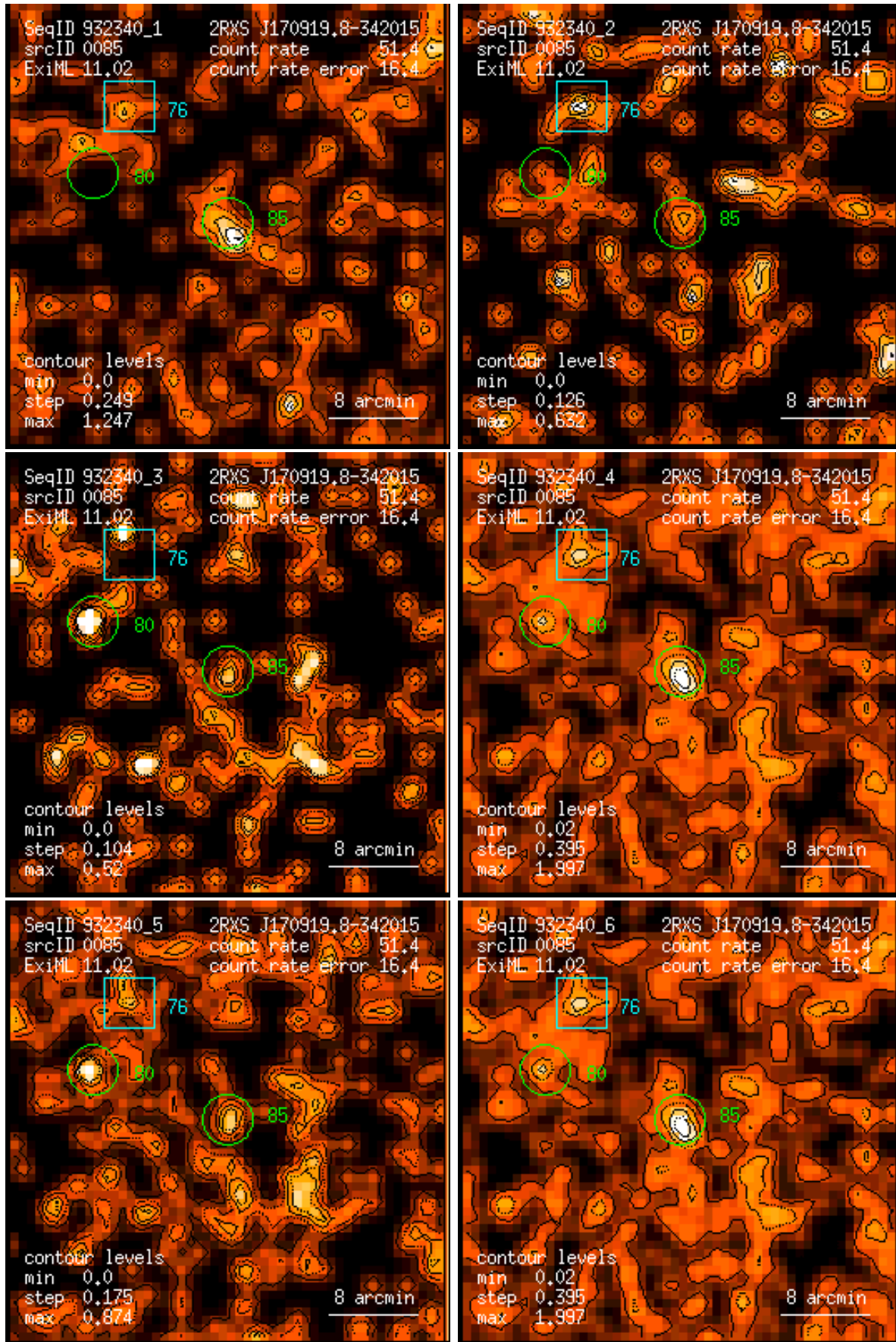
Figure 85: RASS 932340: detection 0085: band rate images, Gaussian filter: (1) PSPC channels 11 – 41, (2) 52 – 90, (3) 91 – 201, (4) 11 – 235, (5) 52 – 201, (6) 11 – 201. Broad band rates in counts/ks. Band rate contour levels in counts/ks/arcmin 2 .
