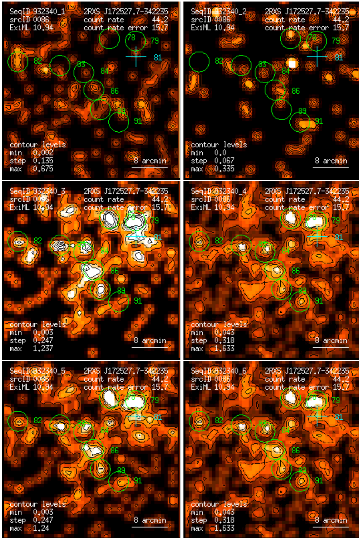
Figure 86: RASS 932340: detection 0086: band rate images, Gaussian filter: (1) PSPC channels 11 – 41, (2) 52 – 90, (3) 91 – 201, (4) 11 – 235, (5) 52 – 201, (6) 11 – 201. Broad band rates in counts/ks. Band rate contour levels in counts/ks/arcmin 2 .
