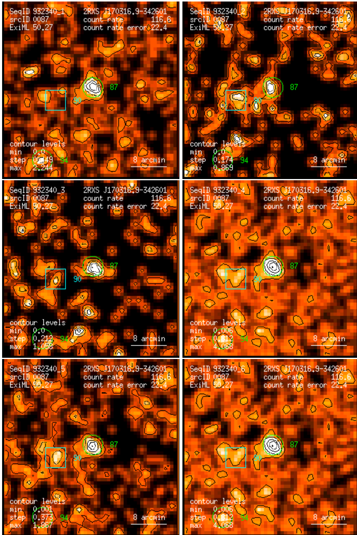
Figure 87: RASS 932340: detection 0087: band rate images, Gaussian filter: (1) PSPC channels 11 – 41, (2) 52 – 90, (3) 91 – 201, (4) 11 – 235, (5) 52 – 201, (6) 11 – 201. Broad band rates in counts/ks. Band rate contour levels in counts/ks/arcmin 2 .
