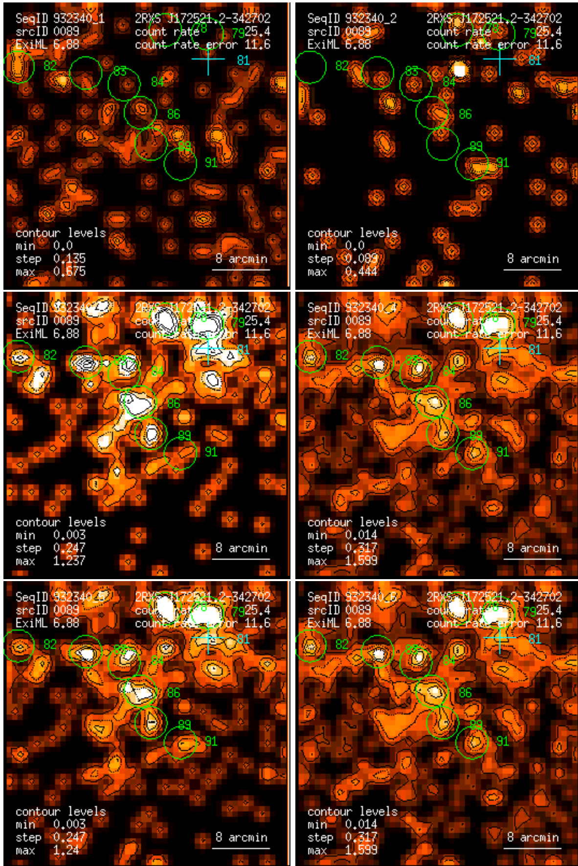
Figure 89: RASS 932340: detection 0089: band rate images, Gaussian filter: (1) PSPC channels 11 – 41, (2) 52 – 90, (3) 91 – 201, (4) 11 – 235, (5) 52 – 201, (6) 11 – 201. Broad band rates in counts/ks. Band rate contour levels in counts/ks/arcmin 2 .
