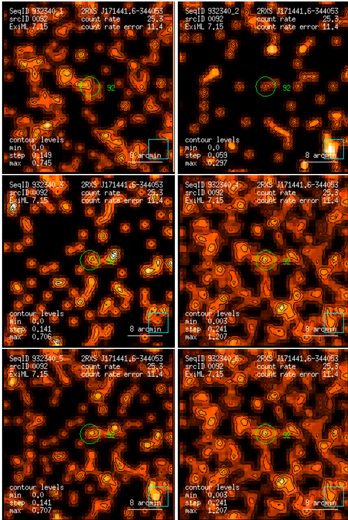
Figure 92: RASS 932340: detection 0092: band rate images, Gaussian filter: (1) PSPC channels 11 – 41, (2) 52 – 90, (3) 91 – 201, (4) 11 – 235, (5) 52 – 201, (6) 11 – 201. Broad band rates in counts/ks. Band rate contour levels in counts/ks/arcmin 2 .
