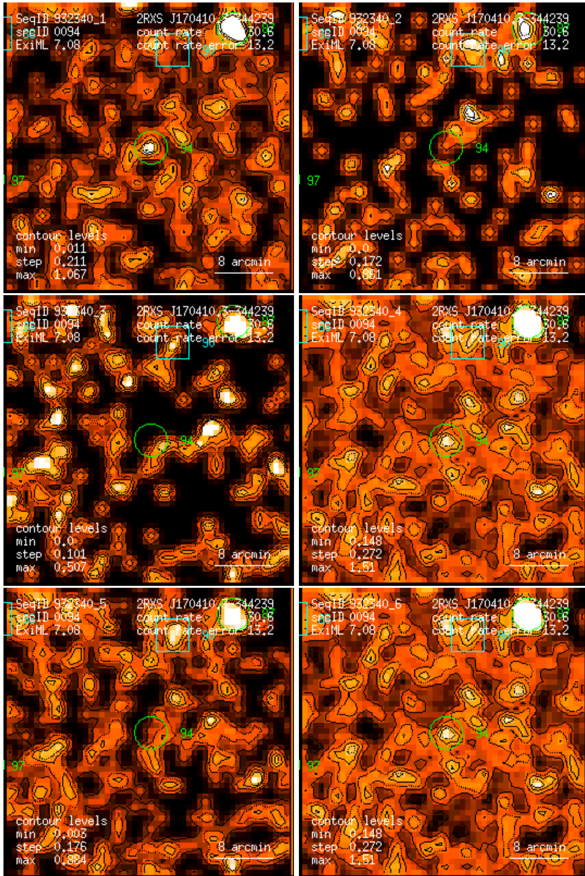
Figure 94: RASS 932340: detection 0094: band rate images, Gaussian filter: (1) PSPC channels 11 – 41, (2) 52 – 90, (3) 91 – 201, (4) 11 – 235, (5) 52 – 201, (6) 11 – 201. Broad band rates in counts/ks. Band rate contour levels in counts/ks/arcmin 2 .
