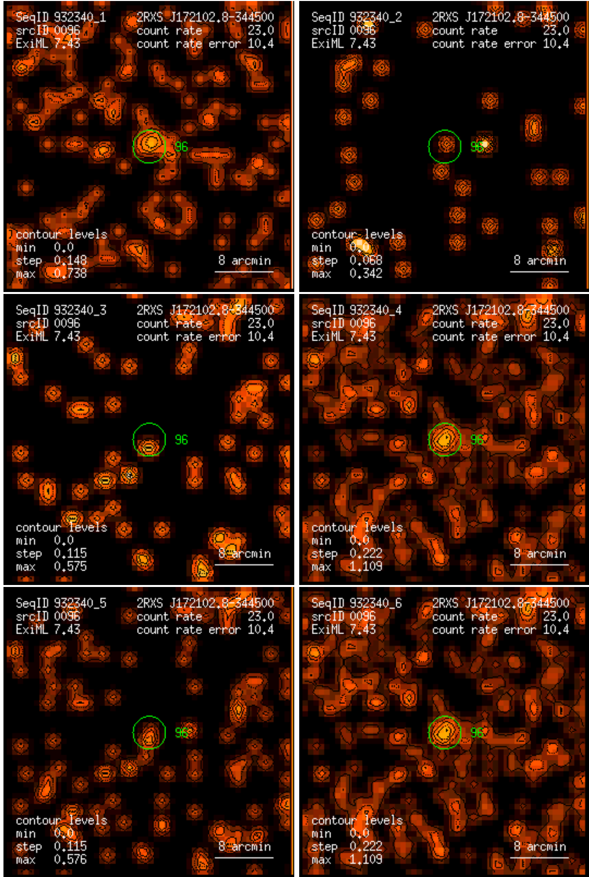
Figure 96: RASS 932340: detection 0096: band rate images, Gaussian filter: (1) PSPC channels 11 – 41, (2) 52 – 90, (3) 91 – 201, (4) 11 – 235, (5) 52 – 201, (6) 11 – 201. Broad band rates in counts/ks. Band rate contour levels in counts/ks/arcmin 2 .
