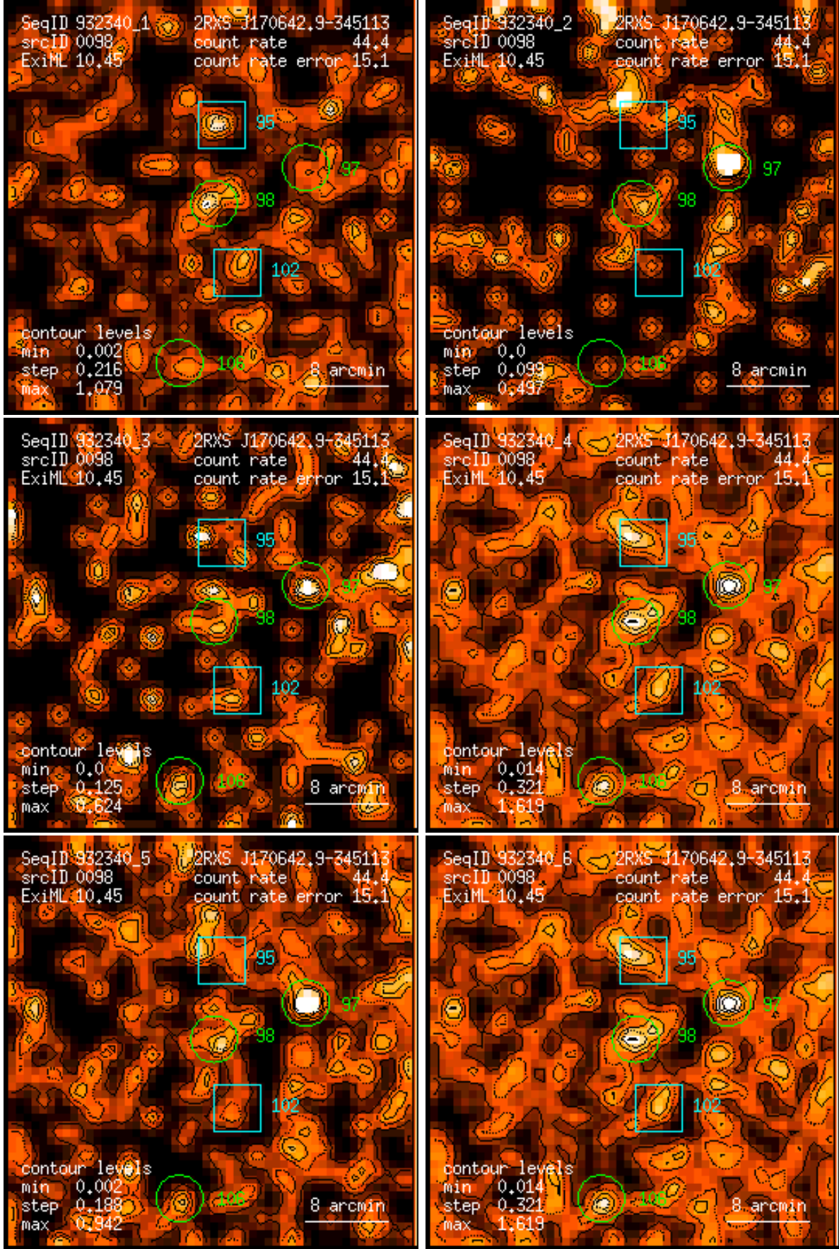
Figure 98: RASS 932340: detection 0098: band rate images, Gaussian filter: (1) PSPC channels 11 – 41, (2) 52 – 90, (3) 91 – 201, (4) 11 – 235, (5) 52 – 201, (6) 11 – 201. Broad band rates in counts/ks. Band rate contour levels in counts/ks/arcmin 2 .
